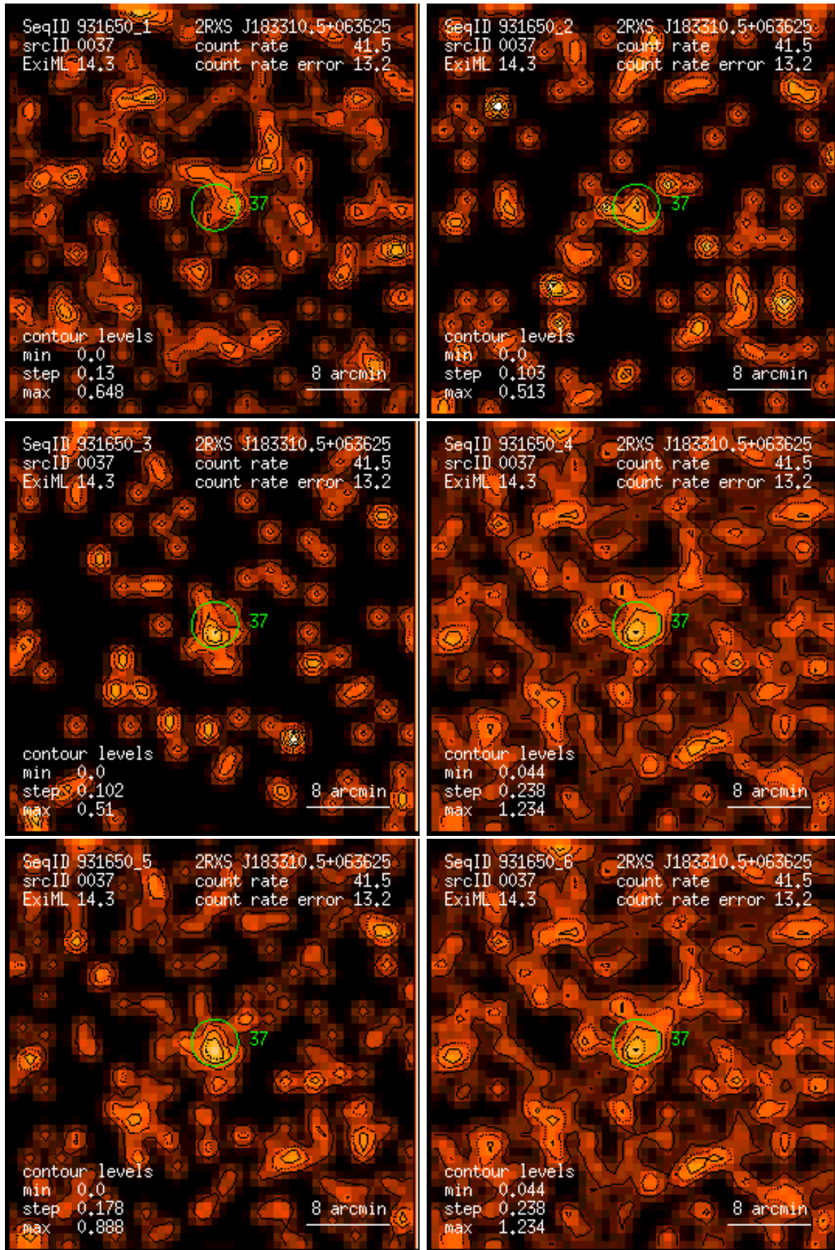
Figure 37: RASS 931650: detection 0037: band rate images, Gaussian filter: (1) PSPC channels 11 – 41, (2) 52 – 90, (3) 91 – 201, (4) 11 – 235, (5) 52 – 201, (6) 11 – 201. Broad band rates in counts/ks. Band rate contour levels in counts/ks/arcmin 2 .
