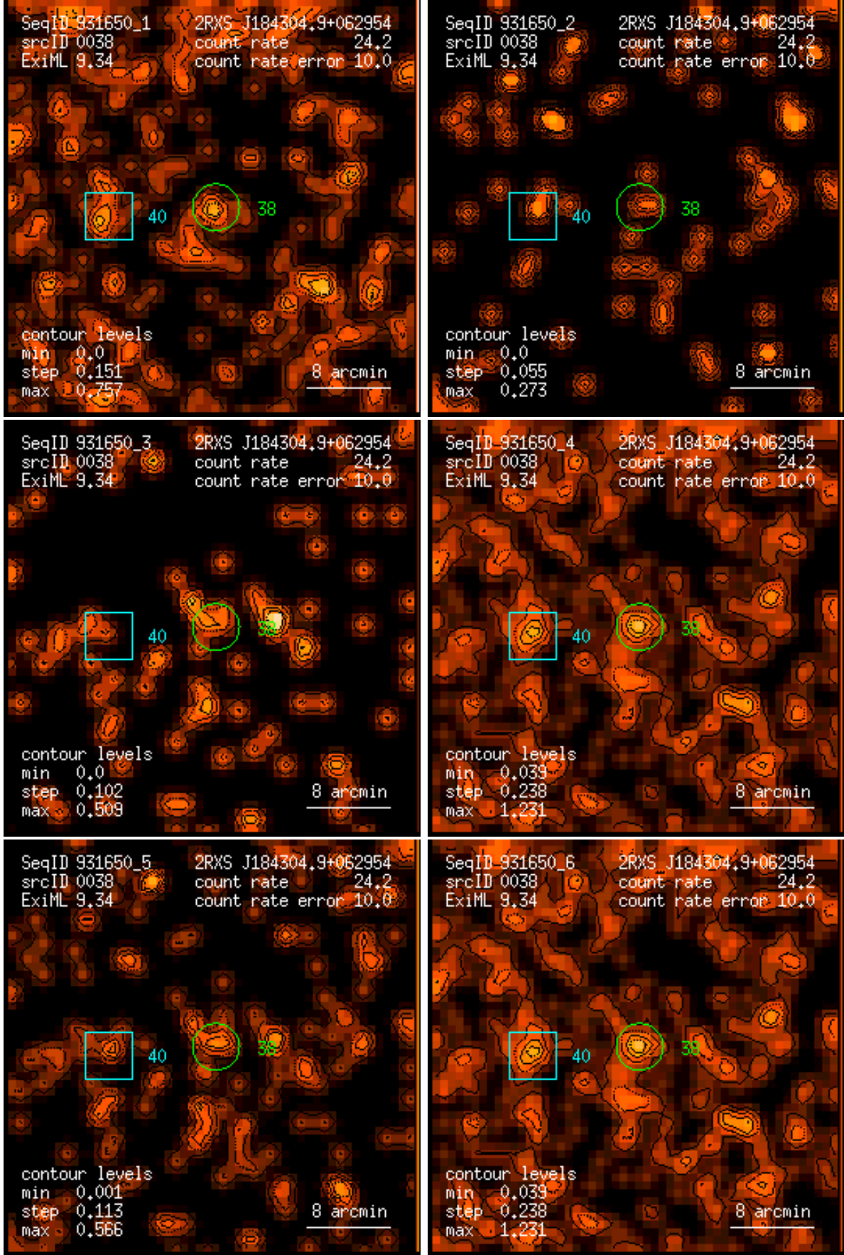
Figure 38: RASS 931650: detection 0038: band rate images, Gaussian filter: (1) PSPC channels 11 – 41, (2) 52 – 90, (3) 91 – 201, (4) 11 – 235, (5) 52 – 201, (6) 11 – 201. Broad band rates in counts/ks. Band rate contour levels in counts/ks/arcmin 2 .
