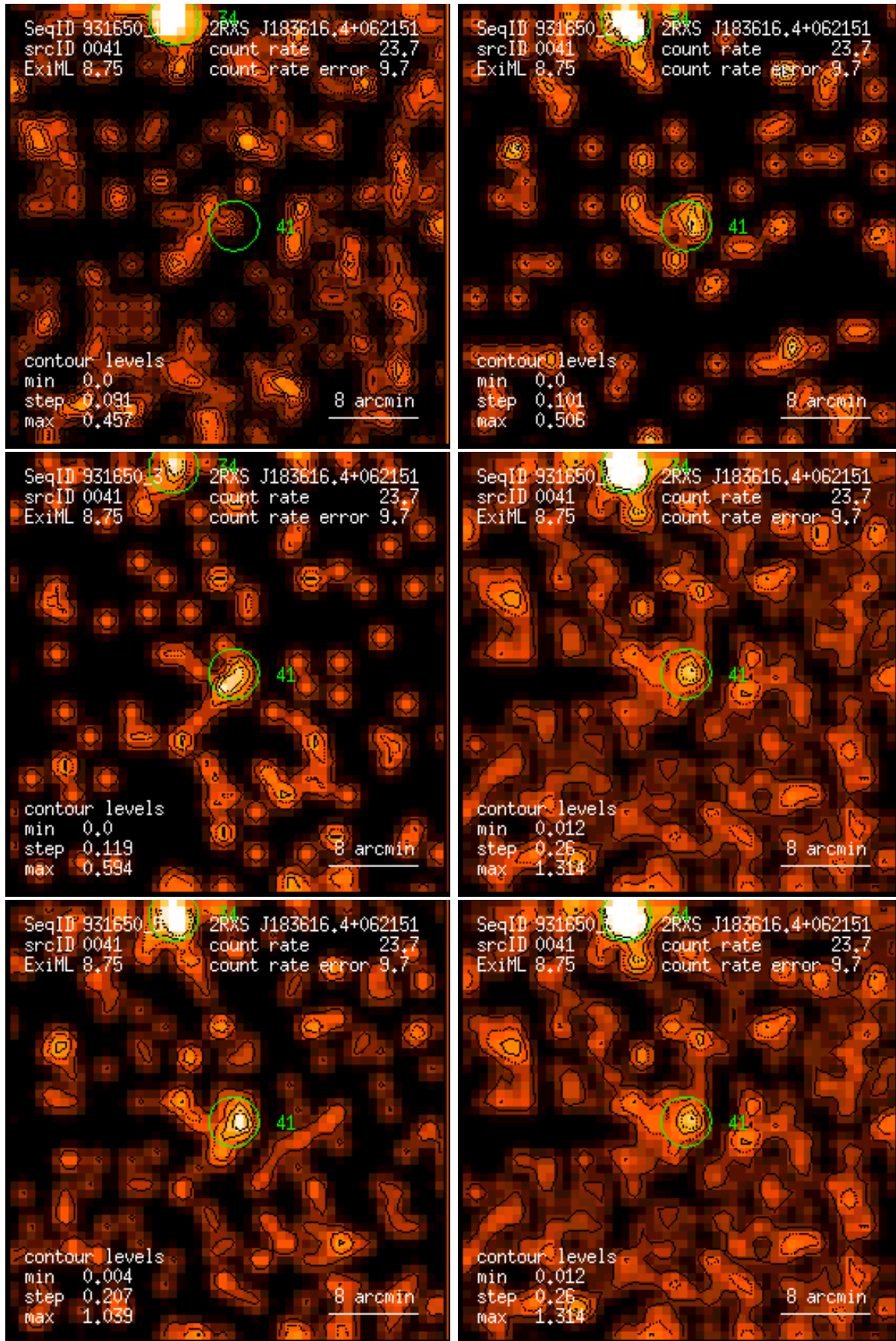
Figure 41: RASS 931650: detection 0041: band rate images, Gaussian filter: (1) PSPC channels 11 – 41, (2) 52 – 90, (3) 91 – 201, (4) 11 – 235, (5) 52 – 201, (6) 11 – 201. Broad band rates in counts/ks. Band rate contour levels in counts/ks/arcmin 2 .
