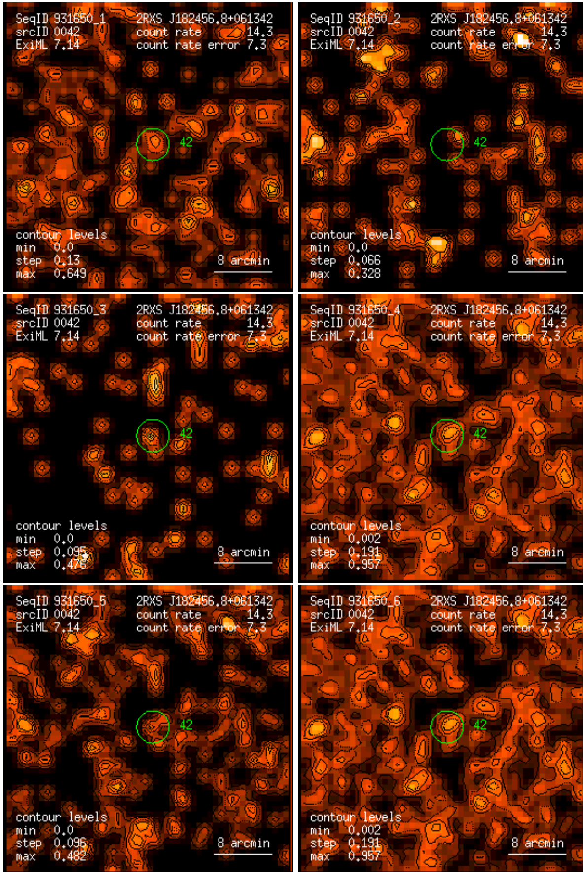
Figure 42: RASS 931650: detection 0042: band rate images, Gaussian filter: (1) PSPC channels 11 – 41, (2) 52 – 90, (3) 91 – 201, (4) 11 – 235, (5) 52 – 201, (6) 11 – 201. Broad band rates in counts/ks. Band rate contour levels in counts/ks/arcmin 2 .
