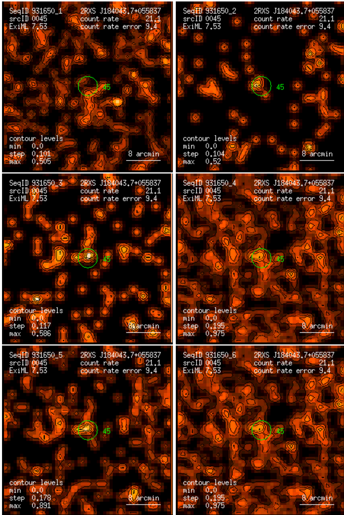
Figure 45: RASS 931650: detection 0045: band rate images, Gaussian filter: (1) PSPC channels 11 – 41, (2) 52 – 90, (3) 91 – 201, (4) 11 – 235, (5) 52 – 201, (6) 11 – 201. Broad band rates in counts/ks. Band rate contour levels in counts/ks/arcmin 2 .
