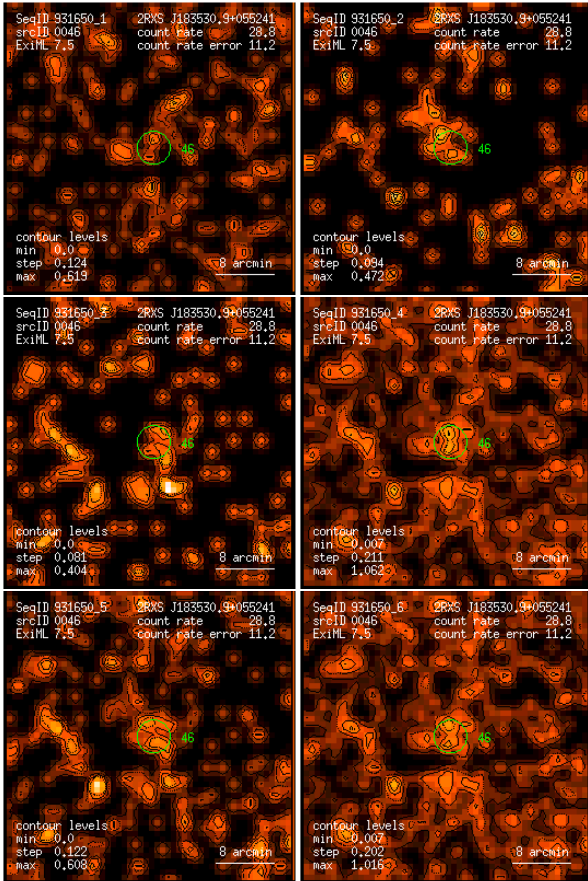
Figure 46: RASS 931650: detection 0046: band rate images, Gaussian filter: (1) PSPC channels 11 – 41, (2) 52 – 90, (3) 91 – 201, (4) 11 – 235, (5) 52 – 201, (6) 11 – 201. Broad band rates in counts/ks. Band rate contour levels in counts/ks/arcmin 2 .
