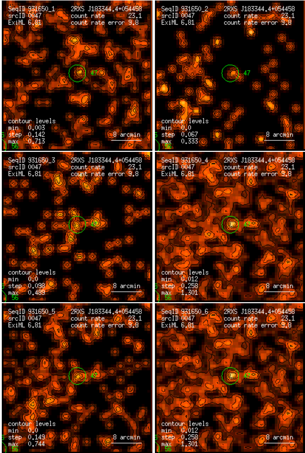
Figure 47: RASS 931650: detection 0047: band rate images, Gaussian filter: (1) PSPC channels 11 – 41, (2) 52 – 90, (3) 91 – 201, (4) 11 – 235, (5) 52 – 201, (6) 11 – 201. Broad band rates in counts/ks. Band rate contour levels in counts/ks/arcmin 2 .
