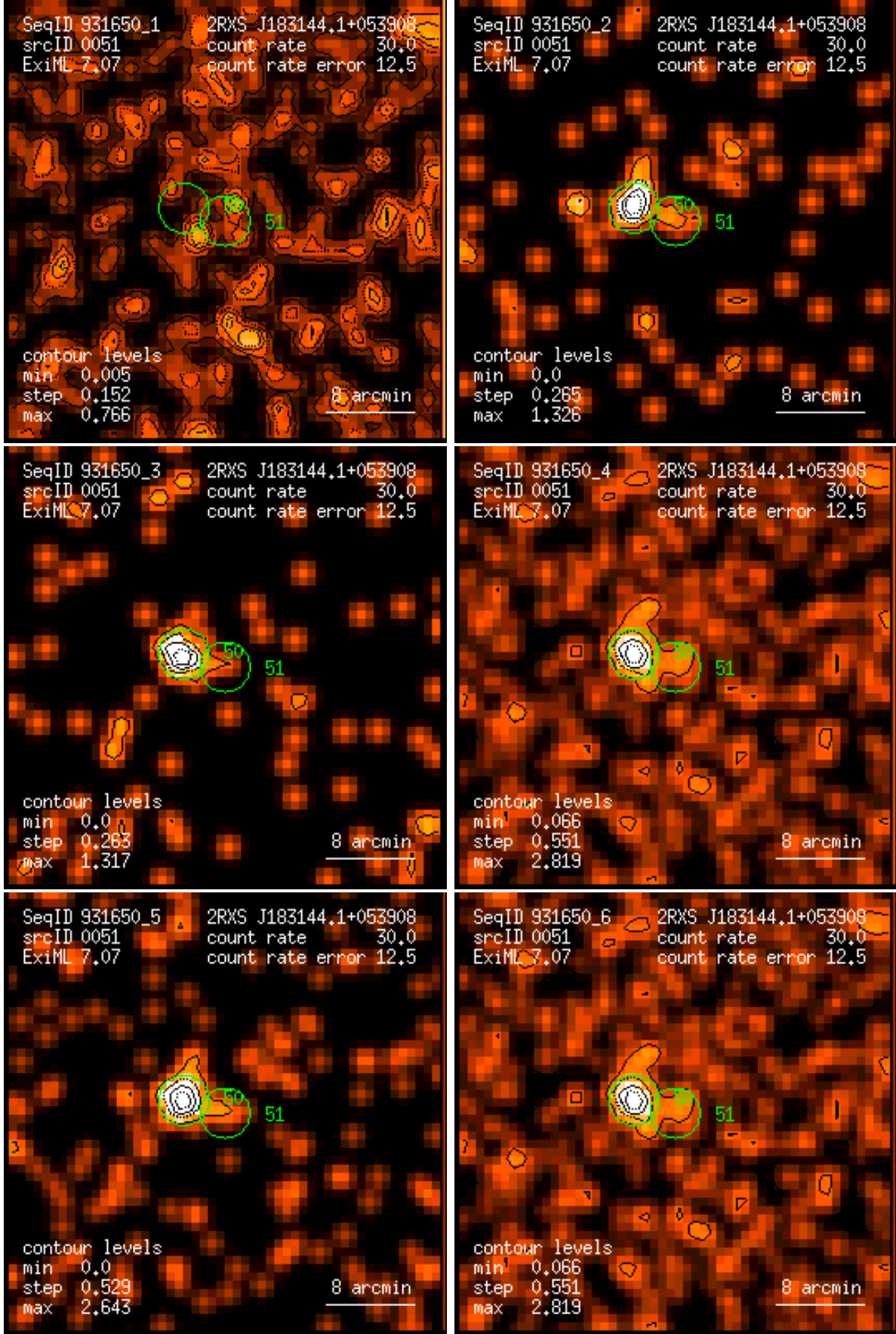
Figure 51: RASS 931650: detection 0051: band rate images, Gaussian filter: (1) PSPC channels 11 – 41, (2) 52 – 90, (3) 91 – 201, (4) 11 – 235, (5) 52 – 201, (6) 11 – 201. Broad band rates in counts/ks. Band rate contour levels in counts/ks/arcmin 2 .
