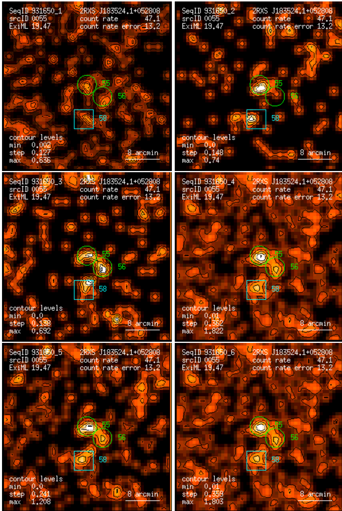
Figure 55: RASS 931650: detection 0055: band rate images, Gaussian filter: (1) PSPC channels 11 – 41, (2) 52 – 90, (3) 91 – 201, (4) 11 – 235, (5) 52 – 201, (6) 11 – 201. Broad band rates in counts/ks. Band rate contour levels in counts/ks/arcmin 2 .
