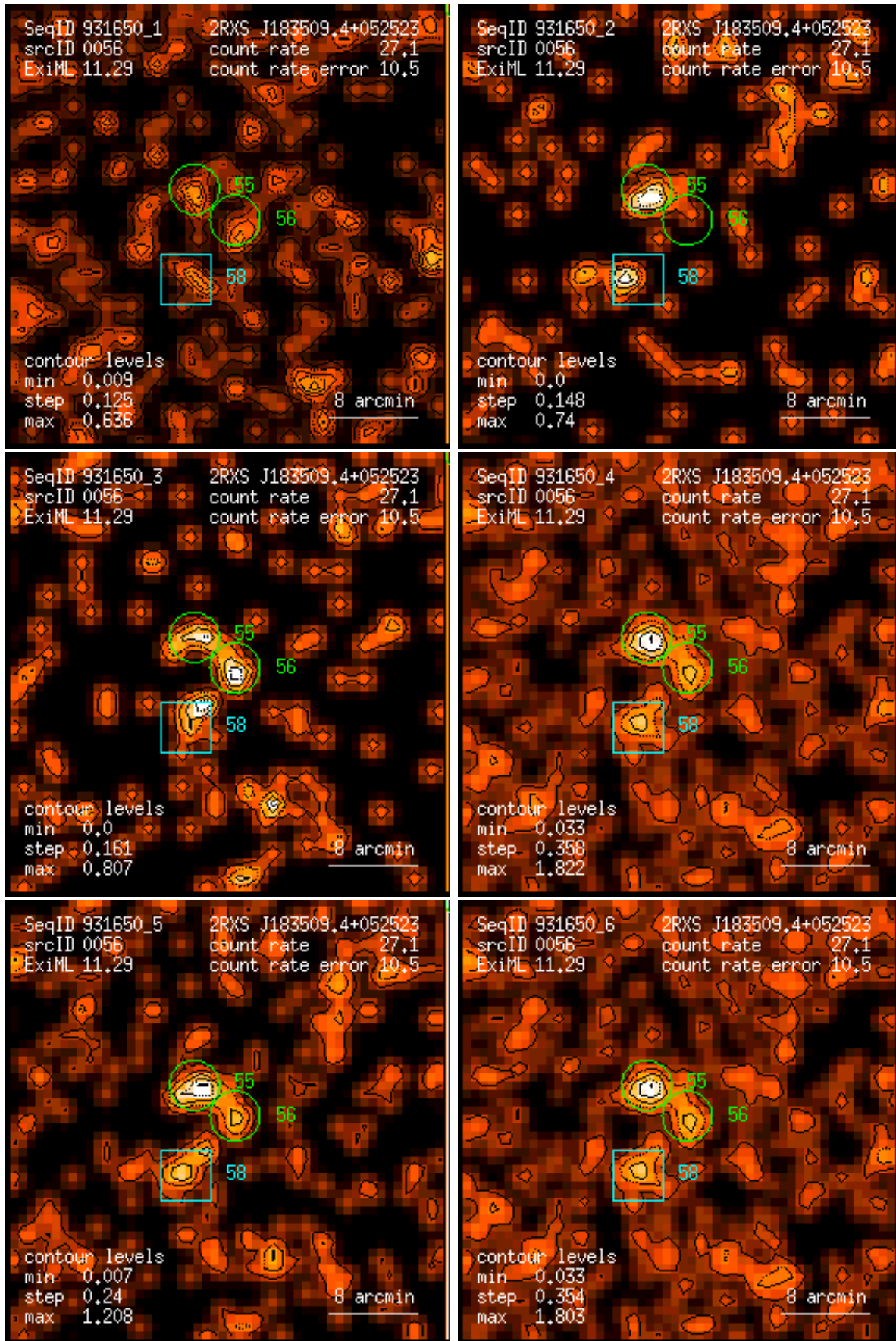
Figure 56: RASS 931650: detection 0056: band rate images, Gaussian filter: (1) PSPC channels 11 – 41, (2) 52 – 90, (3) 91 – 201, (4) 11 – 235, (5) 52 – 201, (6) 11 – 201. Broad band rates in counts/ks. Band rate contour levels in counts/ks/arcmin 2 .
