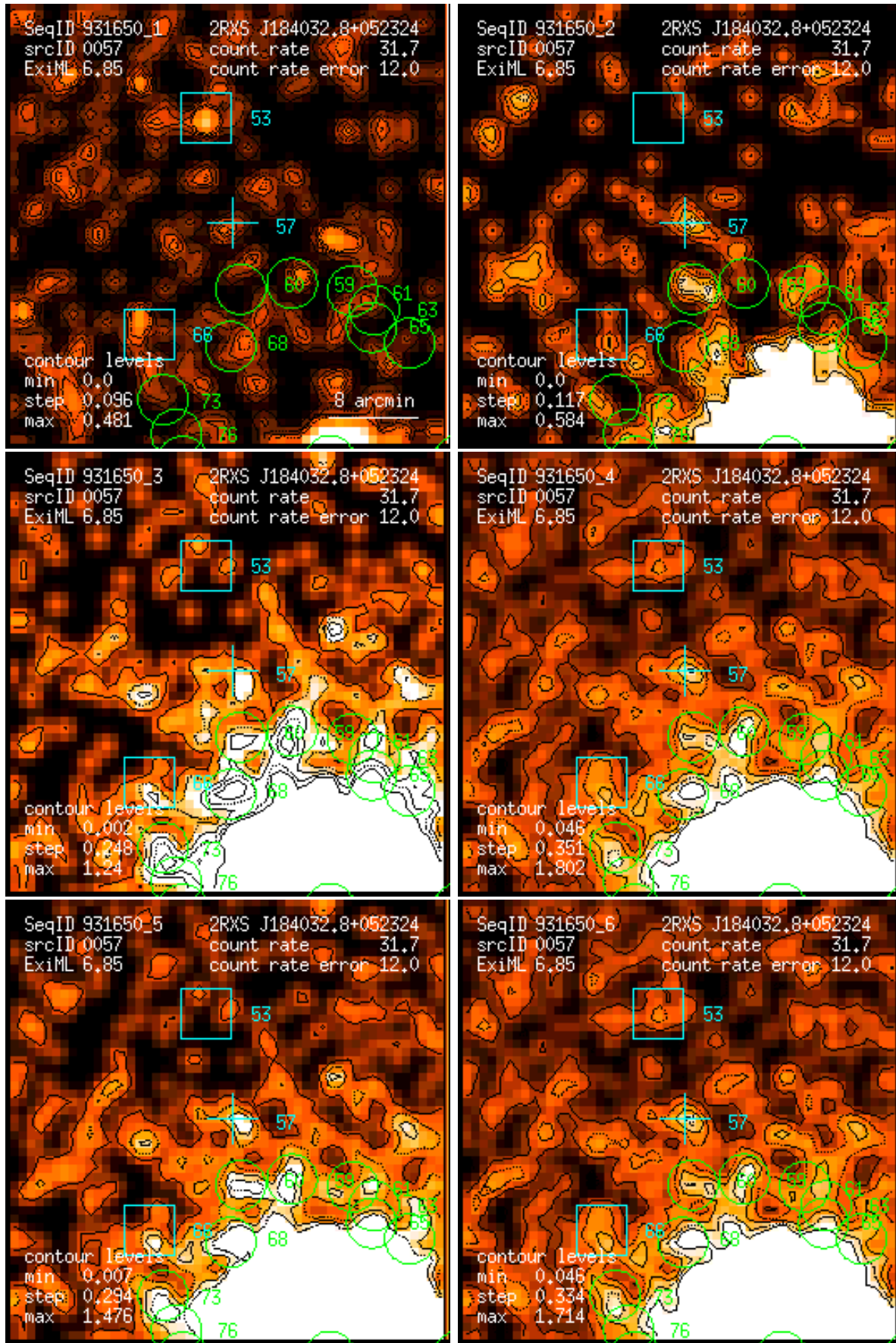
Figure 57: RASS 931650: detection 0057: band rate images, Gaussian filter: (1) PSPC channels 11 – 41, (2) 52 – 90, (3) 91 – 201, (4) 11 – 235, (5) 52 – 201, (6) 11 – 201. Broad band rates in counts/ks. Band rate contour levels in counts/ks/arcmin 2 .
