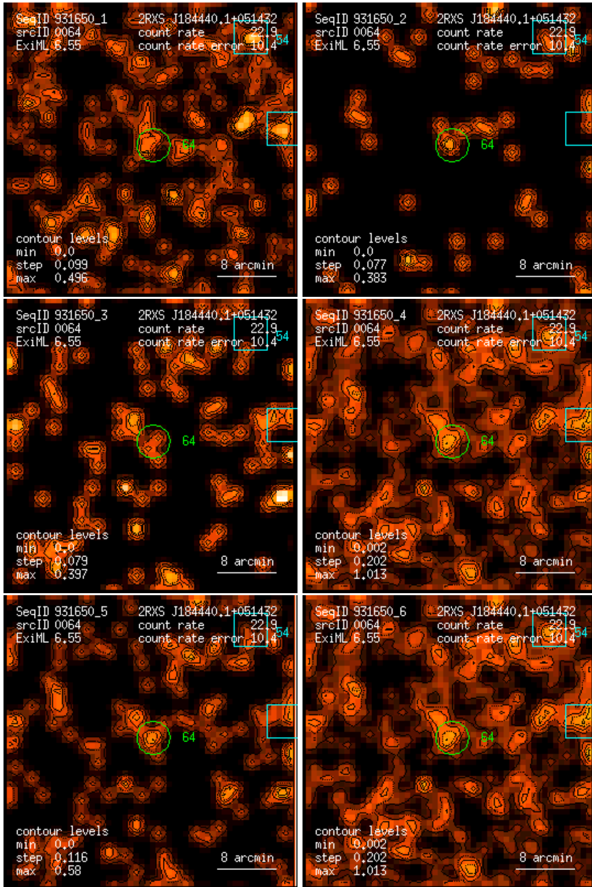
Figure 64: RASS 931650: detection 0064: band rate images, Gaussian filter: (1) PSPC channels 11 – 41, (2) 52 – 90, (3) 91 – 201, (4) 11 – 235, (5) 52 – 201, (6) 11 – 201. Broad band rates in counts/ks. Band rate contour levels in counts/ks/arcmin 2 .
