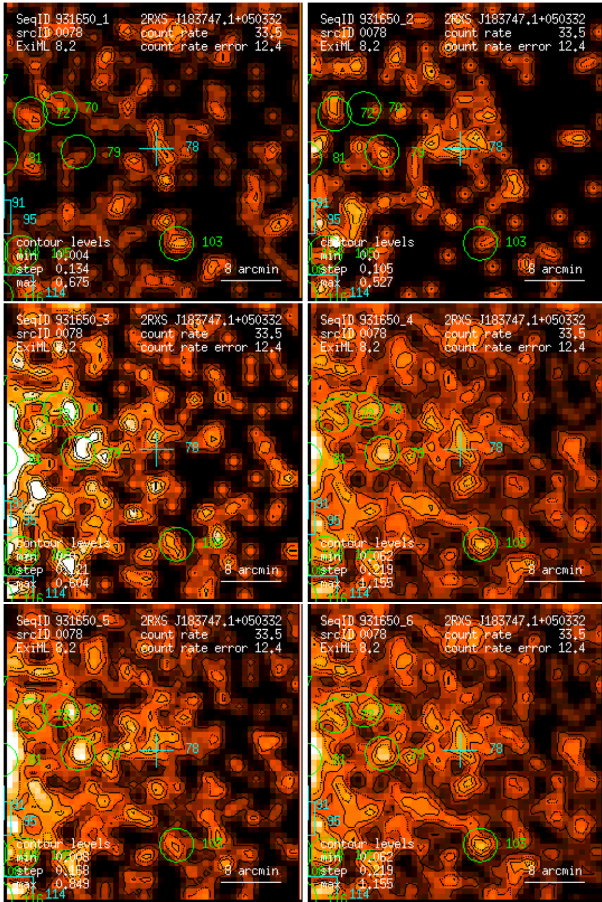
Figure 78: RASS 931650: detection 0078: band rate images, Gaussian filter: (1) PSPC channels 11 – 41, (2) 52 – 90, (3) 91 – 201, (4) 11 – 235, (5) 52 – 201, (6) 11 – 201. Broad band rates in counts/ks. Band rate contour levels in counts/ks/arcmin 2 .
