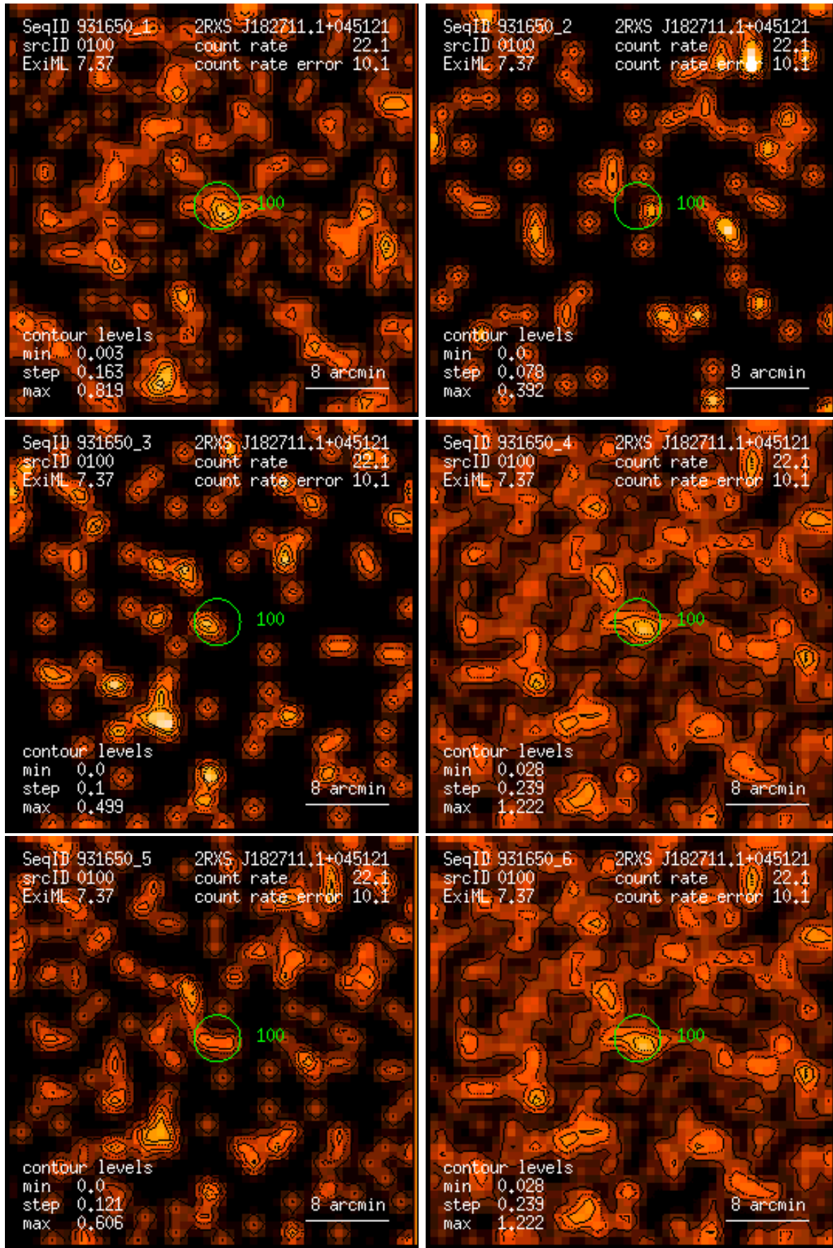
Figure 100: RASS 931650: detection 0100: band rate images, Gaussian filter: (1) PSPC channels 11 – 41, (2) 52 – 90, (3) 91 – 201, (4) 11 – 235, (5) 52 – 201, (6) 11 – 201. Broad band rates in counts/ks. Band rate contour levels in counts/ks/arcmin 2 .
