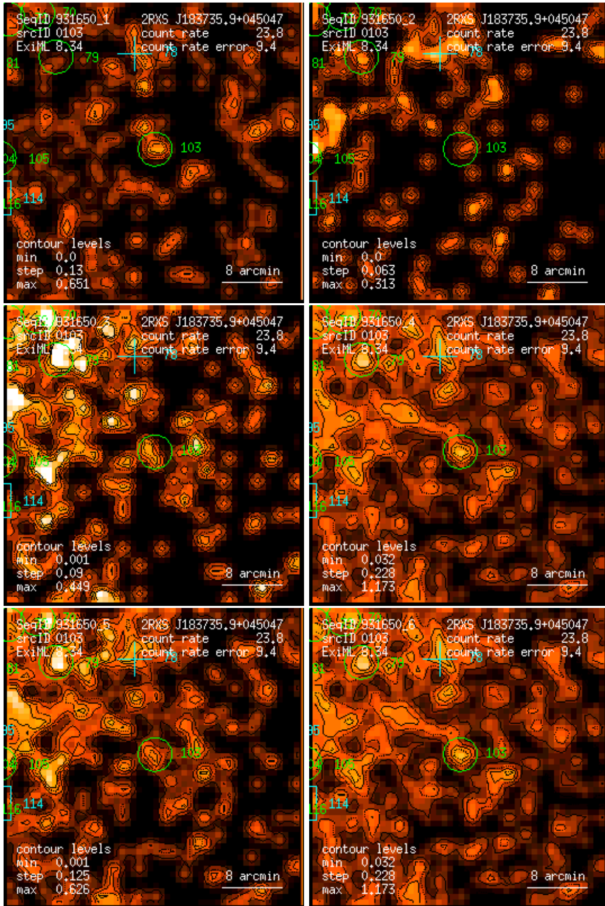
Figure 103: RASS 931650: detection 0103: band rate images, Gaussian filter: (1) PSPC channels 11 – 41, (2) 52 – 90, (3) 91 – 201, (4) 11 – 235, (5) 52 – 201, (6) 11 – 201. Broad band rates in counts/ks. Band rate contour levels in counts/ks/arcmin 2 .
