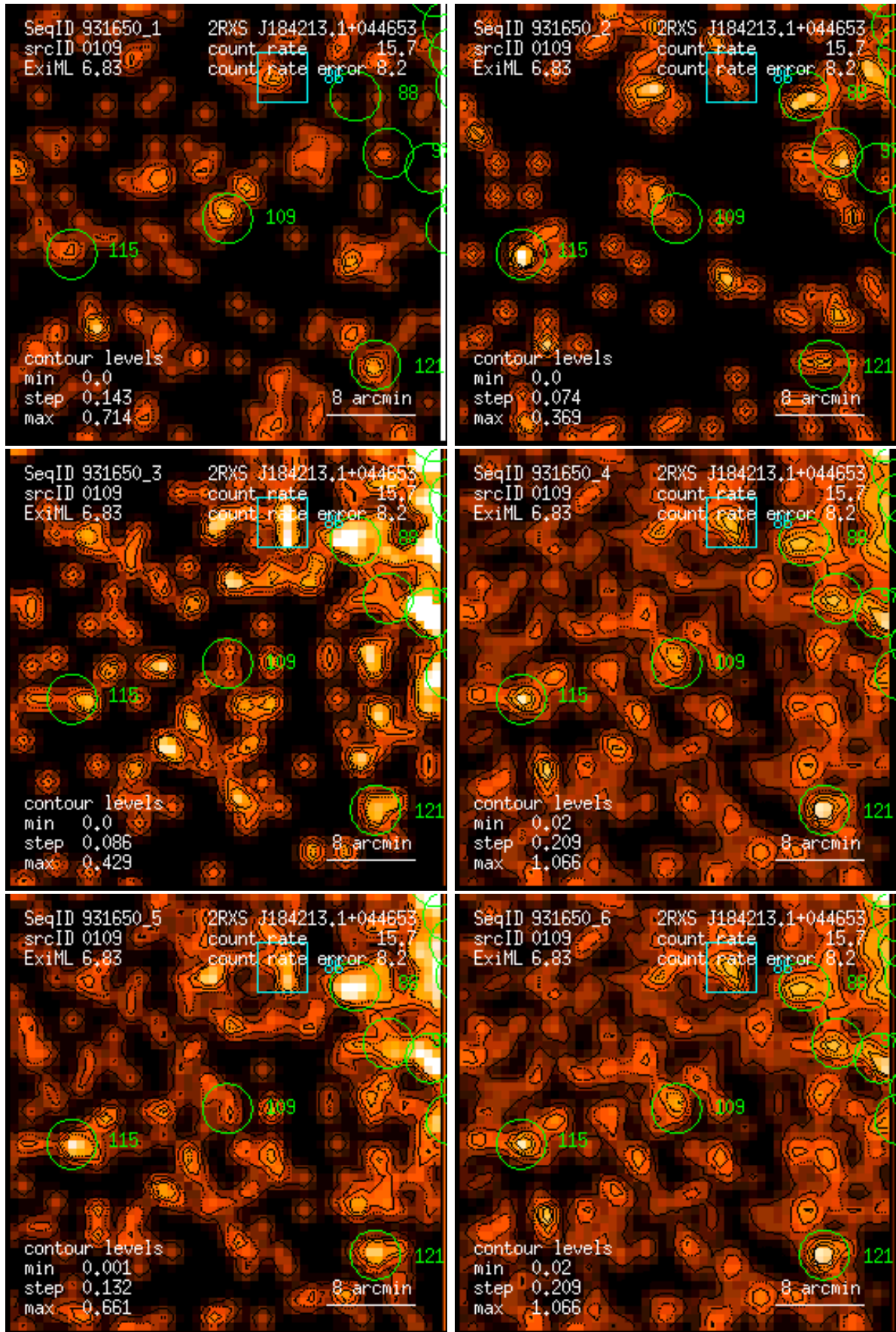
Figure 109: RASS 931650: detection 0109: band rate images, Gaussian filter: (1) PSPC channels 11 – 41, (2) 52 – 90, (3) 91 – 201, (4) 11 – 235, (5) 52 – 201, (6) 11 – 201. Broad band rates in counts/ks. Band rate contour levels in counts/ks/arcmin 2 .
