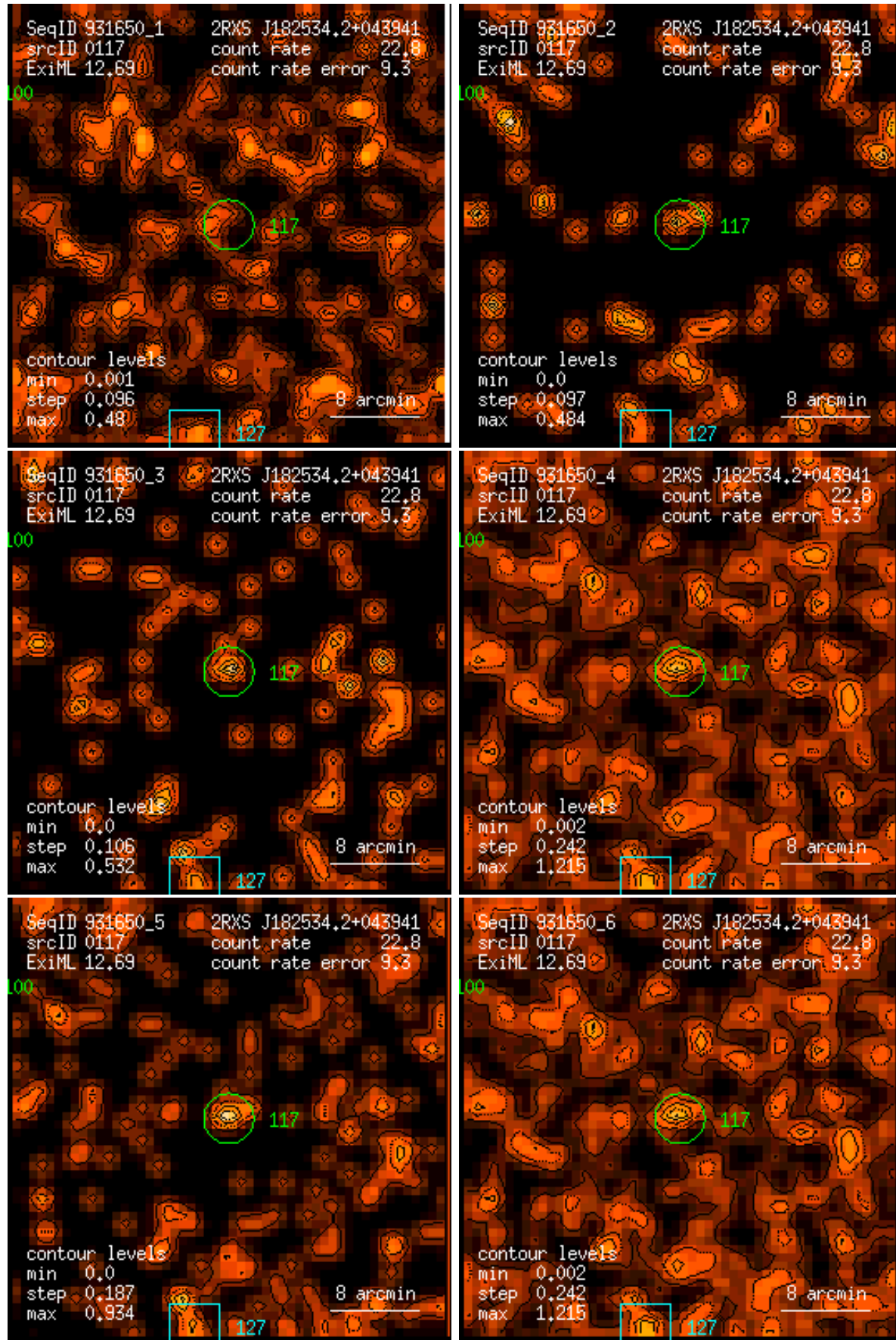
Figure 117: RASS 931650: detection 0117: band rate images, Gaussian filter: (1) PSPC channels 11 – 41, (2) 52 – 90, (3) 91 – 201, (4) 11 – 235, (5) 52 – 201, (6) 11 – 201. Broad band rates in counts/ks. Band rate contour levels in counts/ks/arcmin 2 .
