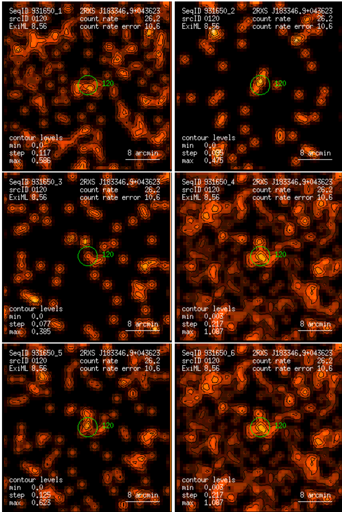
Figure 120: RASS 931650: detection 0120: band rate images, Gaussian filter: (1) PSPC channels 11 – 41, (2) 52 – 90, (3) 91 – 201, (4) 11 – 235, (5) 52 – 201, (6) 11 – 201. Broad band rates in counts/ks. Band rate contour levels in counts/ks/arcmin 2 .
