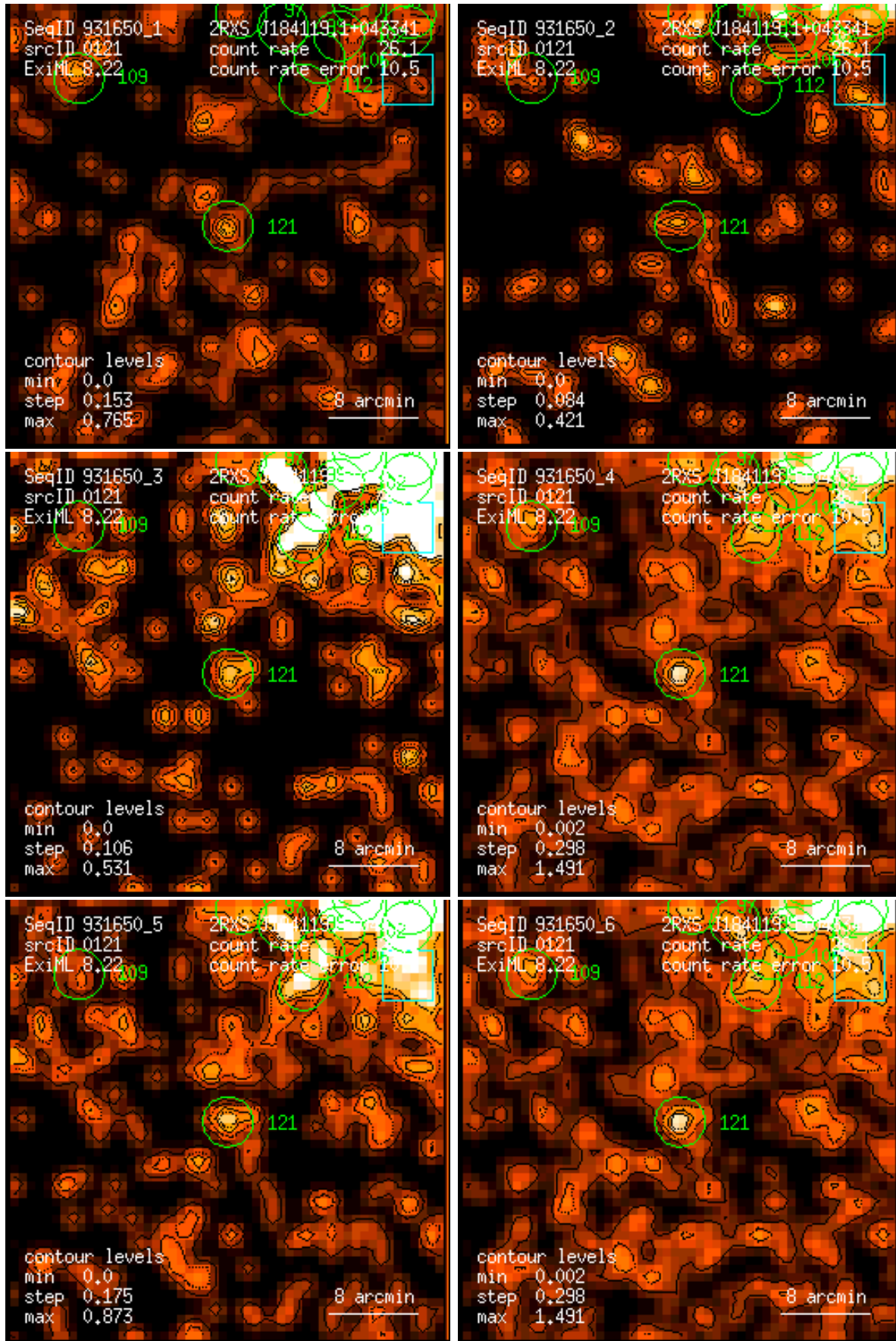
Figure 121: RASS 931650: detection 0121: band rate images, Gaussian filter: (1) PSPC channels 11 – 41, (2) 52 – 90, (3) 91 – 201, (4) 11 – 235, (5) 52 – 201, (6) 11 – 201. Broad band rates in counts/ks. Band rate contour levels in counts/ks/arcmin 2 .
