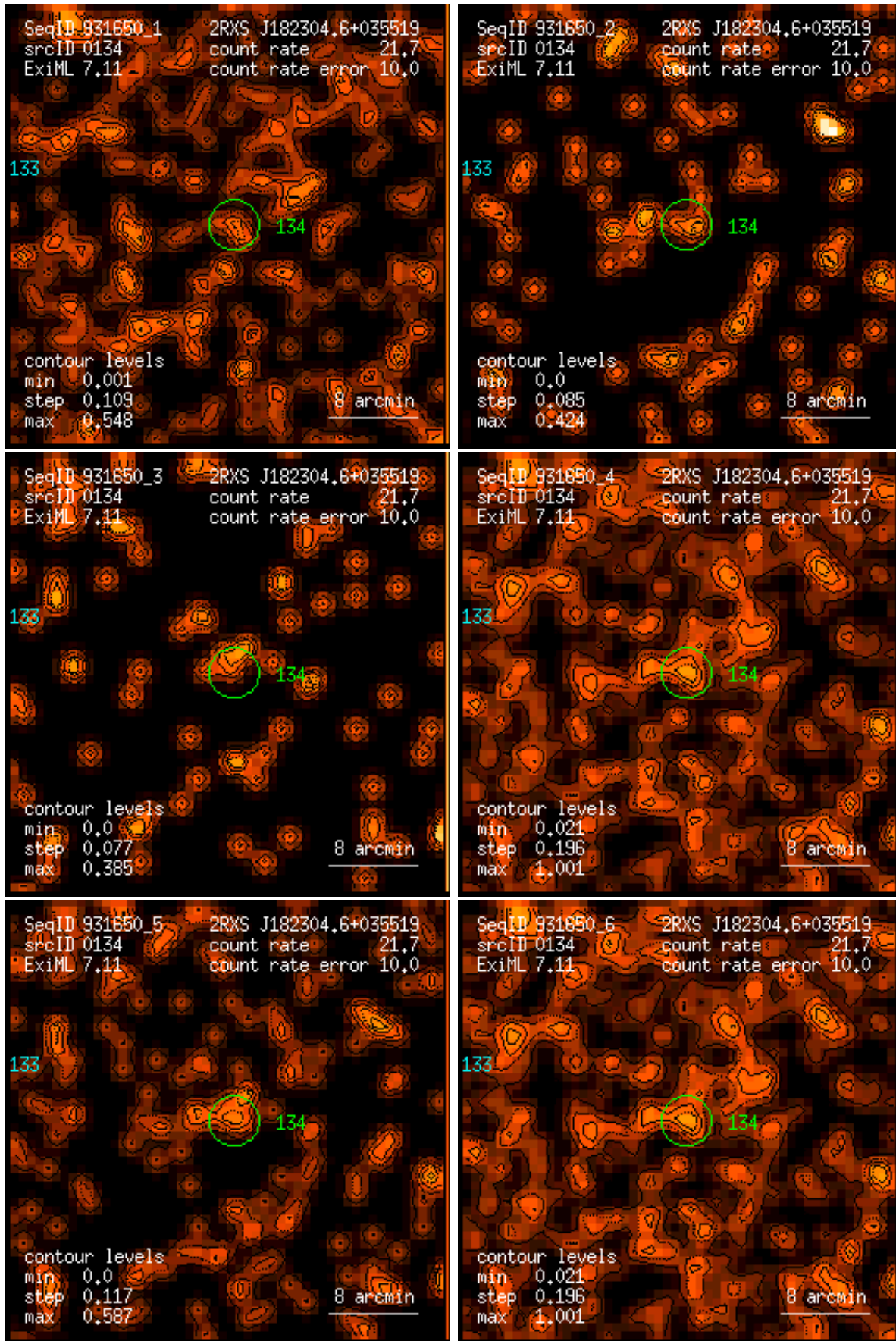
Figure 134: RASS 931650: detection 0134: band rate images, Gaussian filter: (1) PSPC channels 11 – 41, (2) 52 – 90, (3) 91 – 201, (4) 11 – 235, (5) 52 – 201, (6) 11 – 201. Broad band rates in counts/ks. Band rate contour levels in counts/ks/arcmin 2 .
