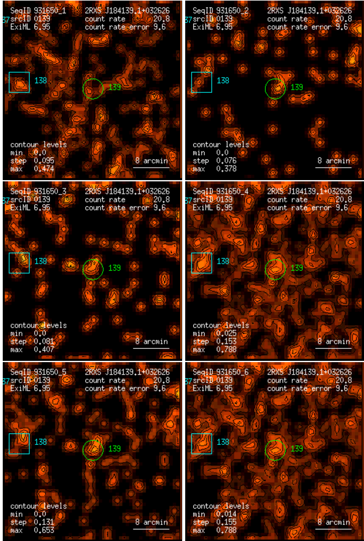
Figure 139: RASS 931650: detection 0139: band rate images, Gaussian filter: (1) PSPC channels 11 – 41, (2) 52 – 90, (3) 91 – 201, (4) 11 – 235, (5) 52 – 201, (6) 11 – 201. Broad band rates in counts/ks. Band rate contour levels in counts/ks/arcmin 2 .
