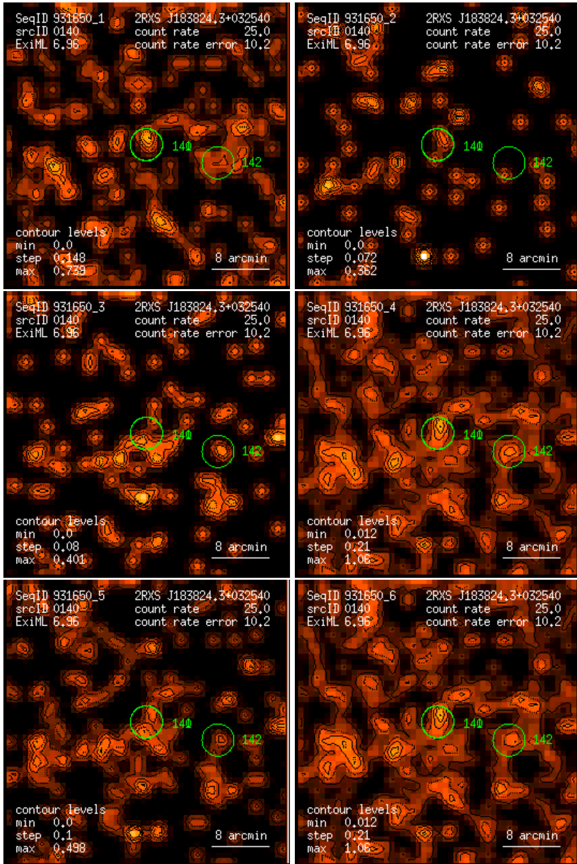
Figure 140: RASS 931650: detection 0140: band rate images, Gaussian filter: (1) PSPC channels 11 – 41, (2) 52 – 90, (3) 91 – 201, (4) 11 – 235, (5) 52 – 201, (6) 11 – 201. Broad band rates in counts/ks. Band rate contour levels in counts/ks/arcmin 2 .
