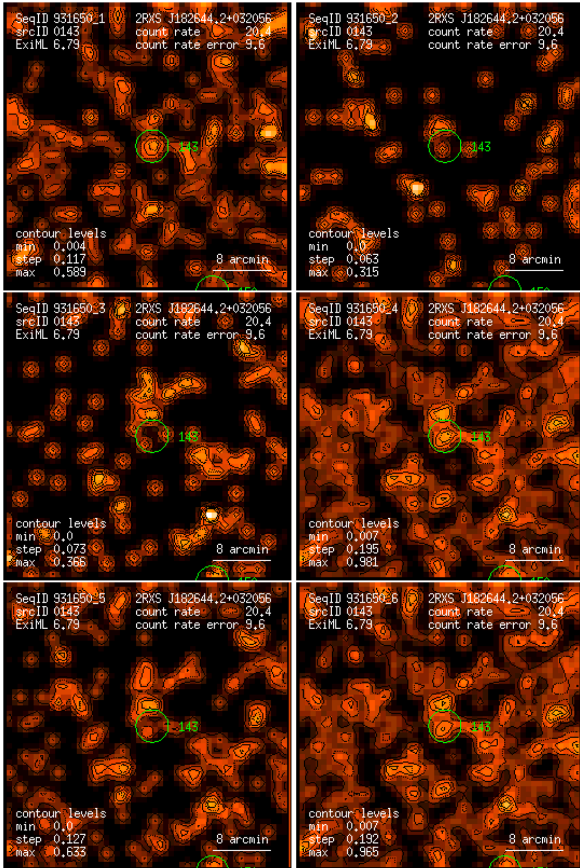
Figure 143: RASS 931650: detection 0143: band rate images, Gaussian filter: (1) PSPC channels 11 – 41, (2) 52 – 90, (3) 91 – 201, (4) 11 – 235, (5) 52 – 201, (6) 11 – 201. Broad band rates in counts/ks. Band rate contour levels in counts/ks/arcmin 2 .
