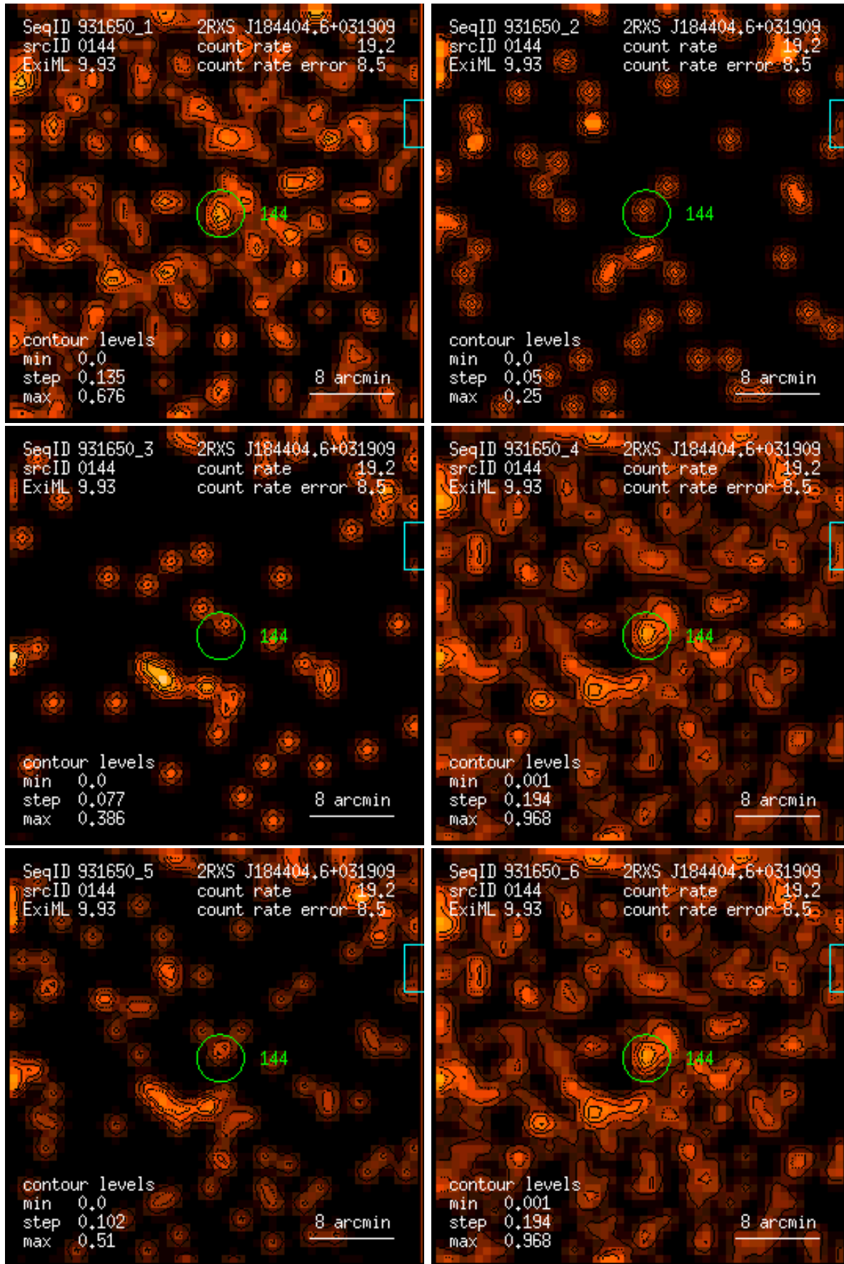
Figure 144: RASS 931650: detection 0144: band rate images, Gaussian filter: (1) PSPC channels 11 – 41, (2) 52 – 90, (3) 91 – 201, (4) 11 – 235, (5) 52 – 201, (6) 11 – 201. Broad band rates in counts/ks. Band rate contour levels in counts/ks/arcmin 2 .
