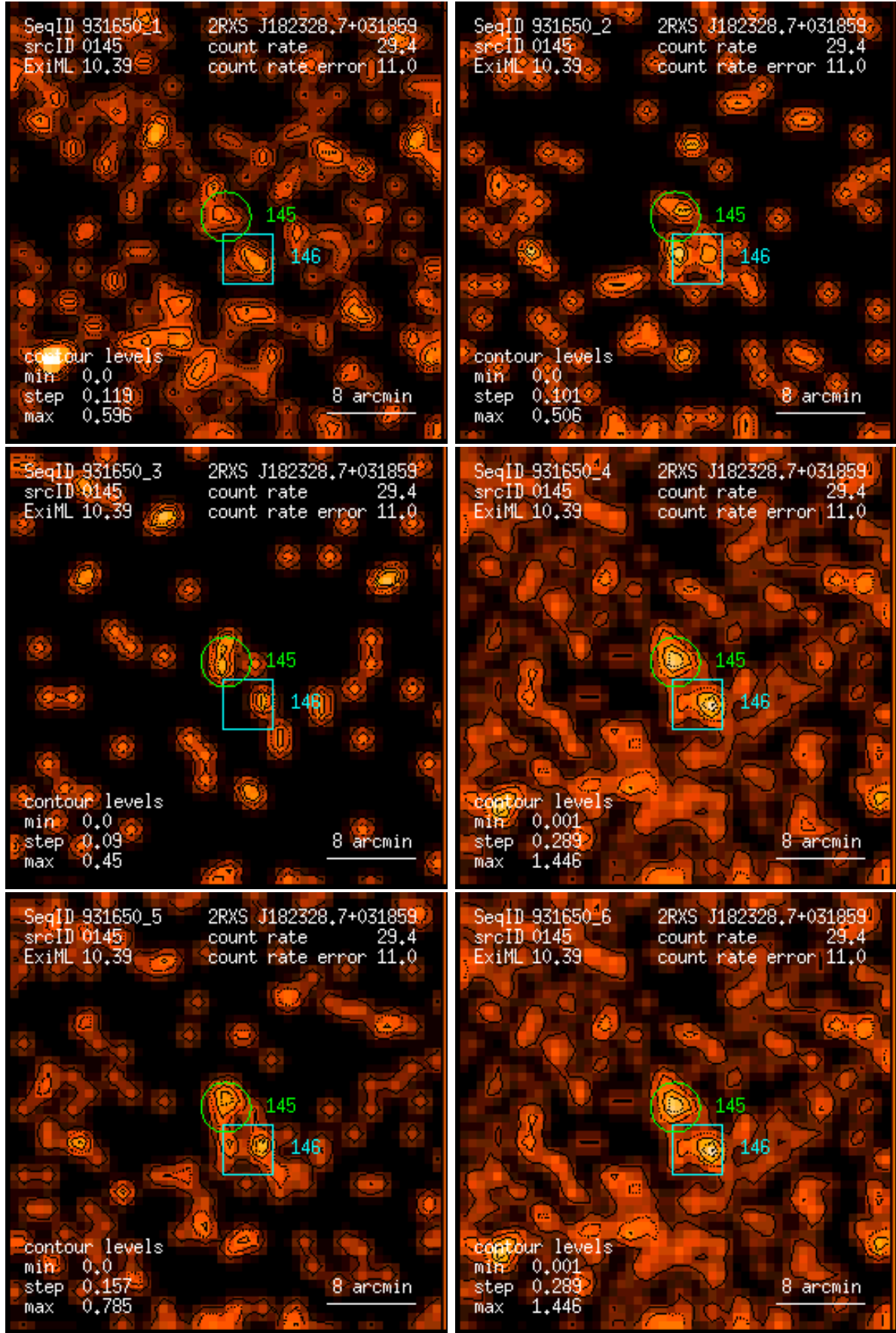
Figure 145: RASS 931650: detection 0145: band rate images, Gaussian filter: (1) PSPC channels 11 – 41, (2) 52 – 90, (3) 91 – 201, (4) 11 – 235, (5) 52 – 201, (6) 11 – 201. Broad band rates in counts/ks. Band rate contour levels in counts/ks/arcmin 2 .
