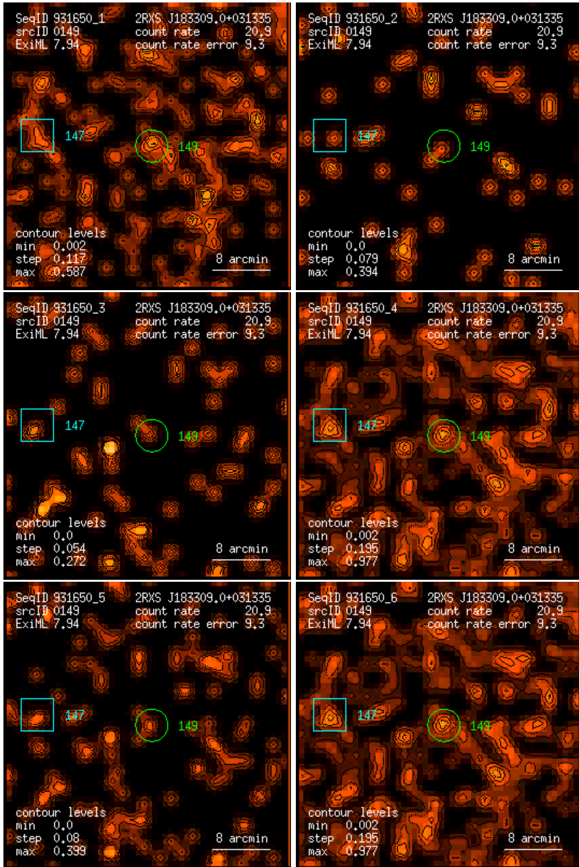
Figure 149: RASS 931650: detection 0149: band rate images, Gaussian filter: (1) PSPC channels 11 – 41, (2) 52 – 90, (3) 91 – 201, (4) 11 – 235, (5) 52 – 201, (6) 11 – 201. Broad band rates in counts/ks. Band rate contour levels in counts/ks/arcmin 2 .
