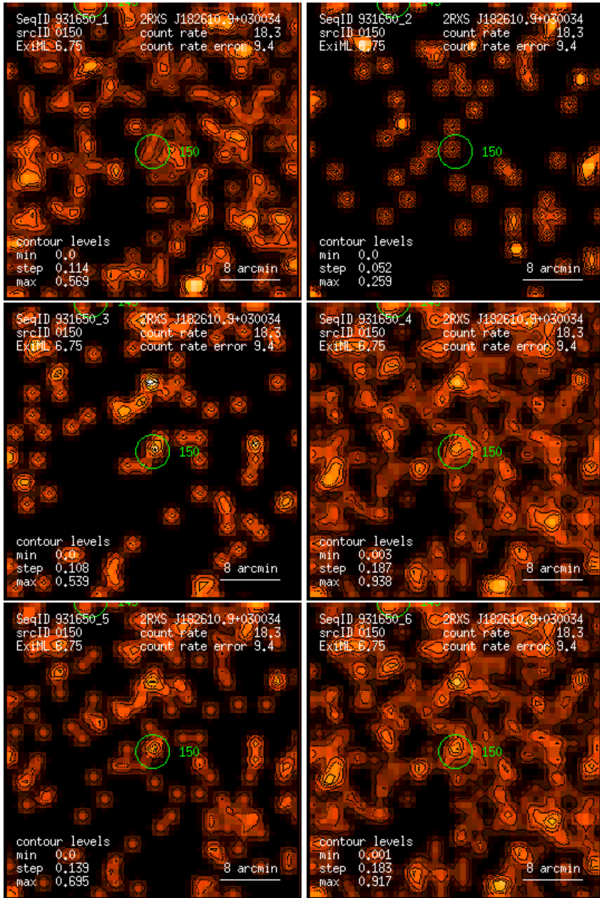
Figure 150: RASS 931650: detection 0150: band rate images, Gaussian filter: (1) PSPC channels 11 – 41, (2) 52 – 90, (3) 91 – 201, (4) 11 – 235, (5) 52 – 201, (6) 11 – 201. Broad band rates in counts/ks. Band rate contour levels in counts/ks/arcmin 2 .
