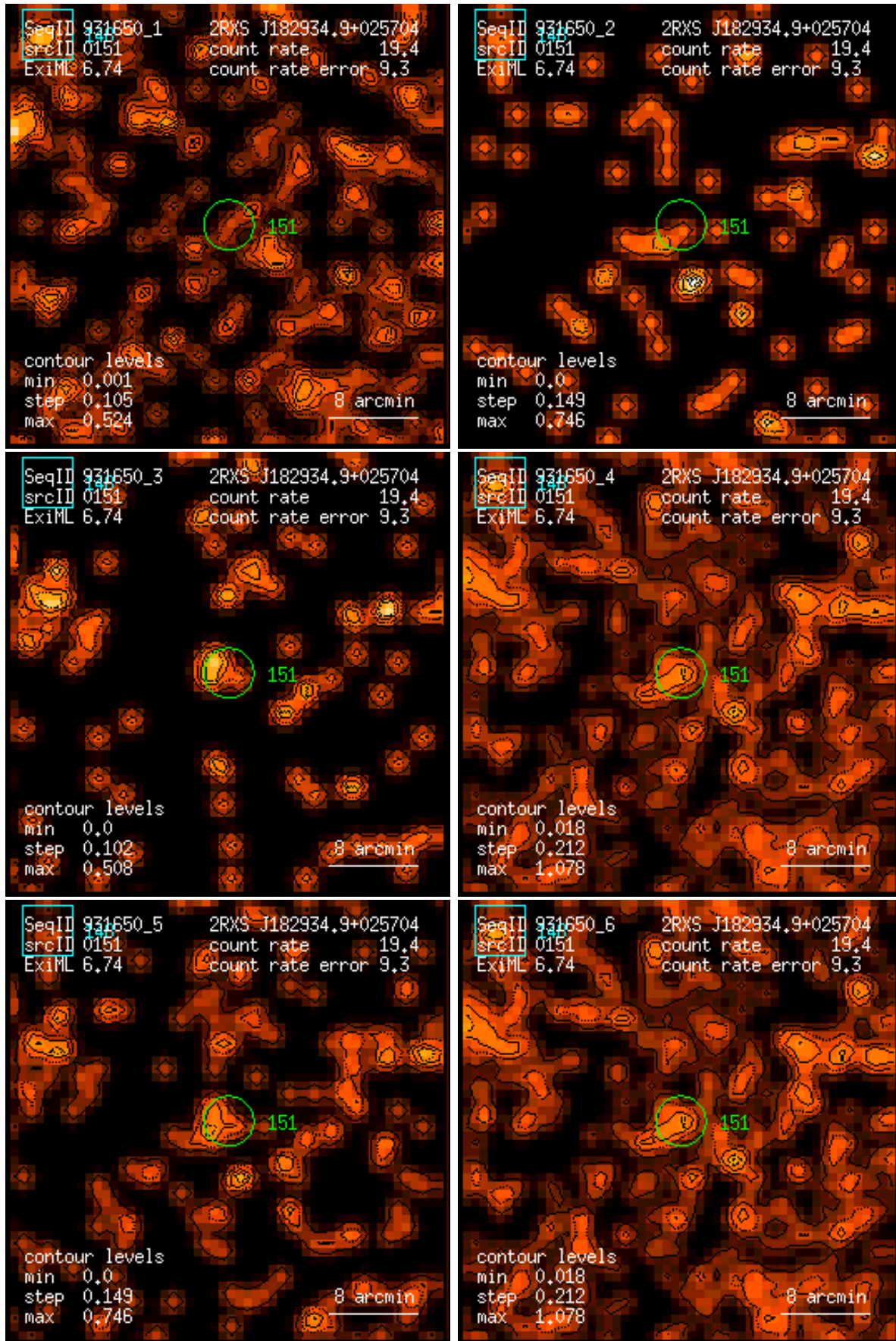
Figure 151: RASS 931650: detection 0151: band rate images, Gaussian filter: (1) PSPC channels 11 – 41, (2) 52 – 90, (3) 91 – 201, (4) 11 – 235, (5) 52 – 201, (6) 11 – 201. Broad band rates in counts/ks. Band rate contour levels in counts/ks/arcmin 2 .
