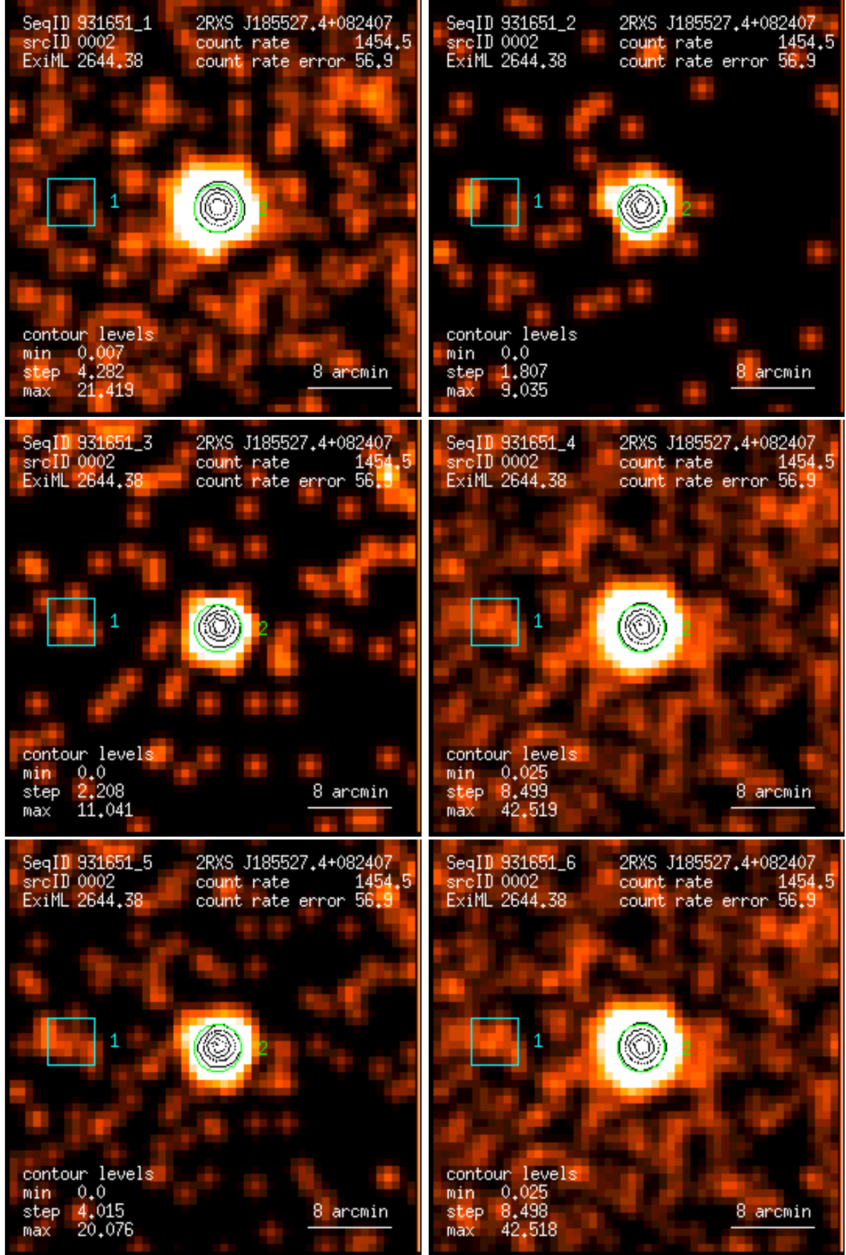
Figure 2: RASS 931651: detection 0002: band rate images, Gaussian filter: (1) PSPC channels 11 – 41, (2) 52 – 90, (3) 91 – 201, (4) 11 – 235, (5) 52 – 201, (6) 11 – 201. Broad band rates in counts/ks. Band rate contour levels in counts/ks/arcmin 2 .
