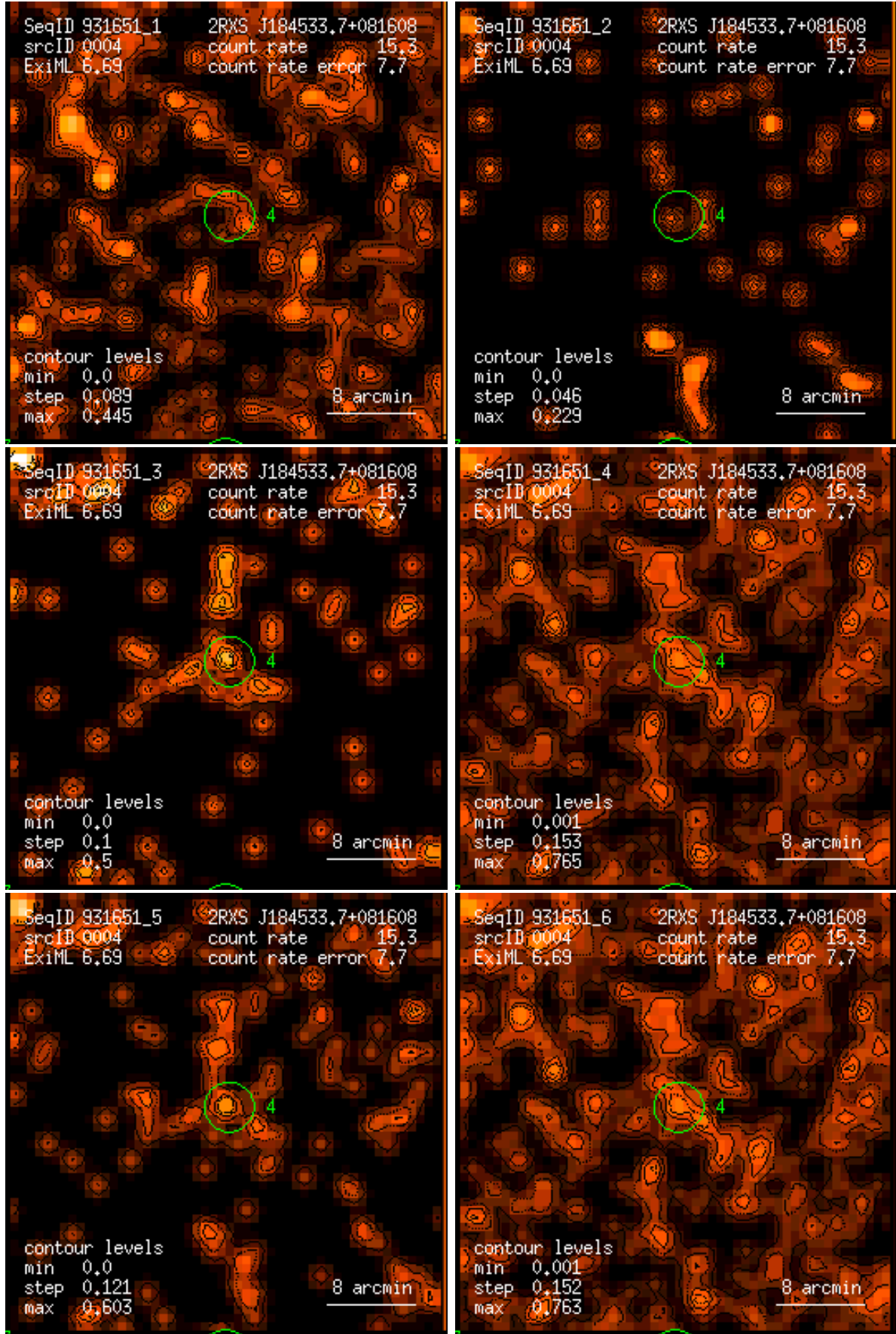
Figure 4: RASS 931651: detection 0004: band rate images, Gaussian filter: (1) PSPC channels 11 – 41, (2) 52 – 90, (3) 91 – 201, (4) 11 – 235, (5) 52 – 201, (6) 11 – 201. Broad band rates in counts/ks. Band rate contour levels in counts/ks/arcmin 2 .
