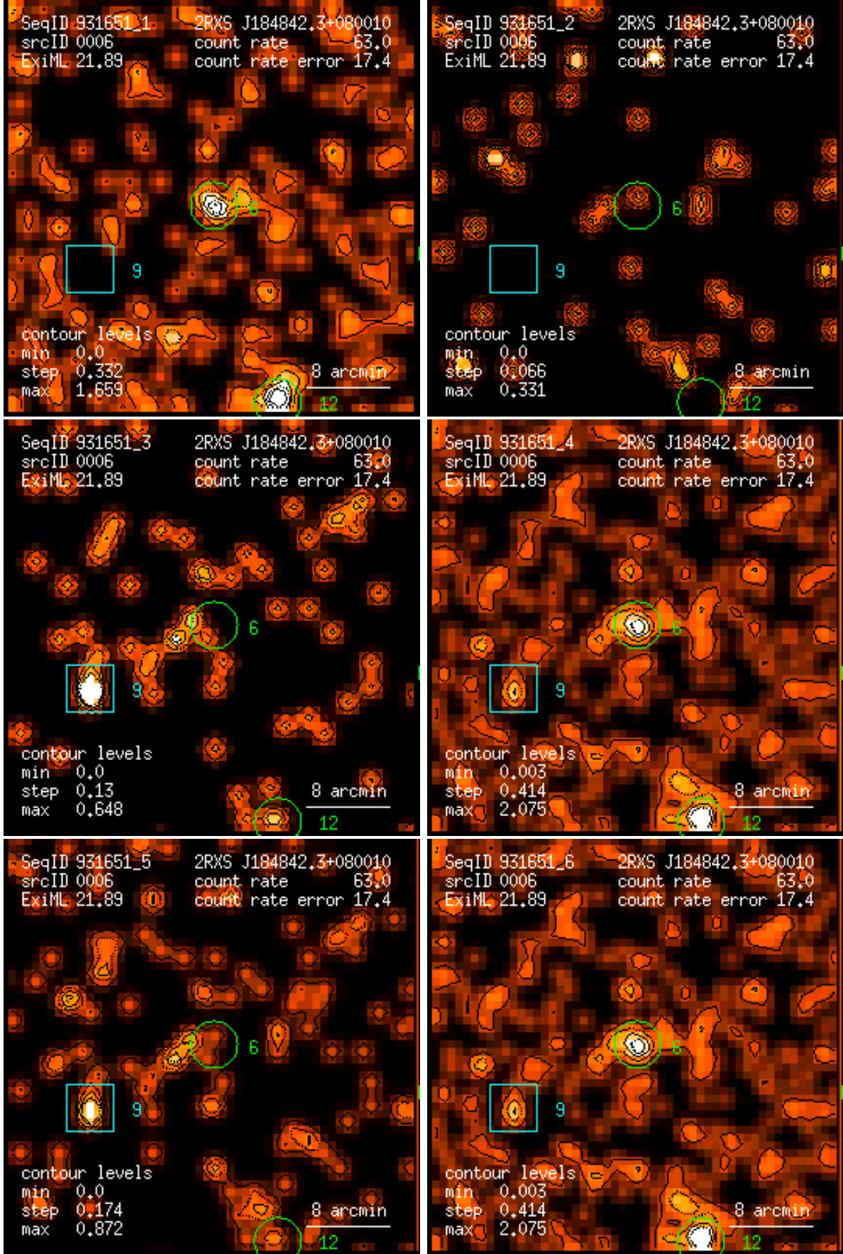
Figure 6: RASS 931651: detection 0006: band rate images, Gaussian filter: (1) PSPC channels 11 – 41, (2) 52 – 90, (3) 91 – 201, (4) 11 – 235, (5) 52 – 201, (6) 11 – 201. Broad band rates in counts/ks. Band rate contour levels in counts/ks/arcmin 2 .
