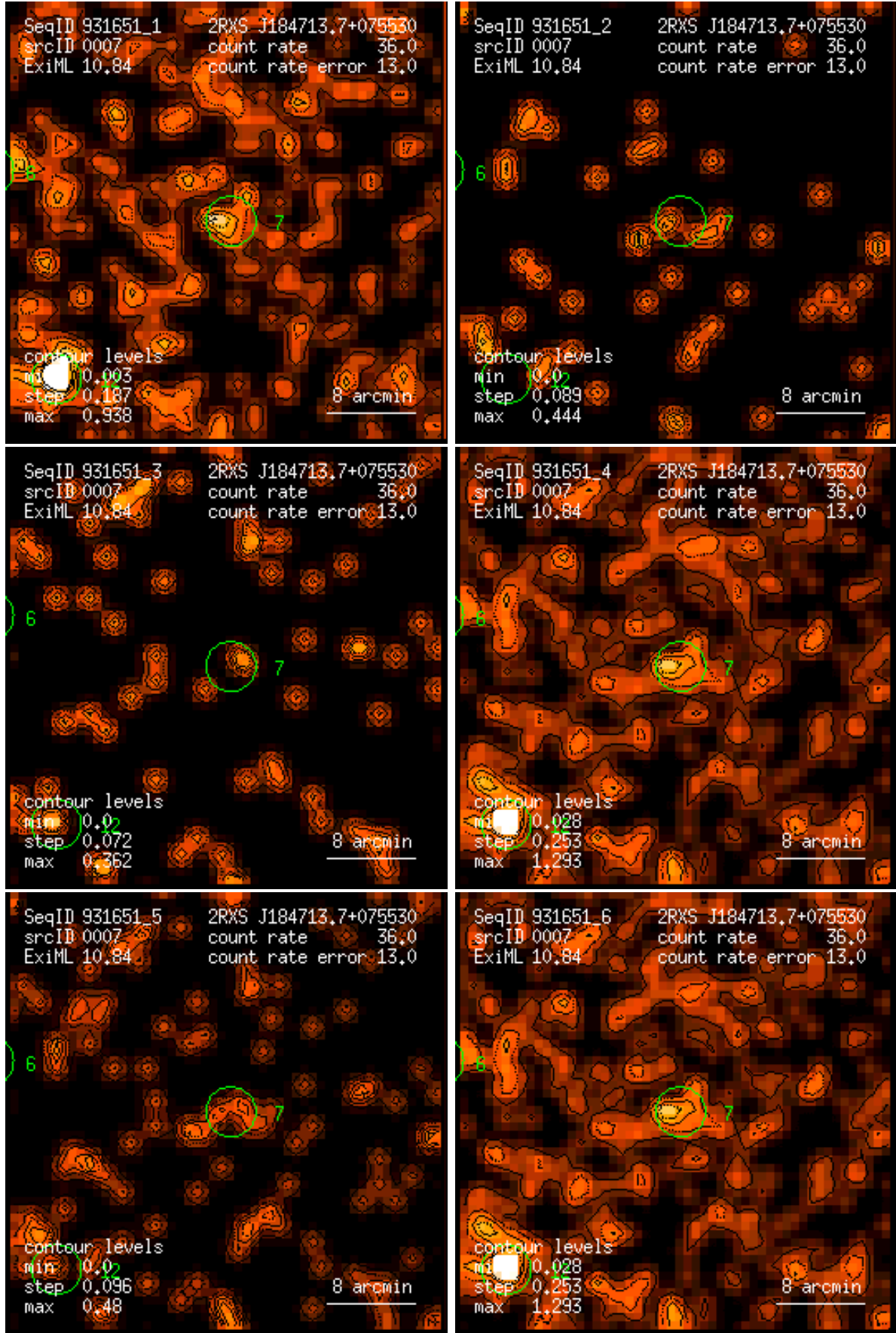
Figure 7: RASS 931651: detection 0007: band rate images, Gaussian filter: (1) PSPC channels 11 – 41, (2) 52 – 90, (3) 91 – 201, (4) 11 – 235, (5) 52 – 201, (6) 11 – 201. Broad band rates in counts/ks. Band rate contour levels in counts/ks/arcmin 2 .
