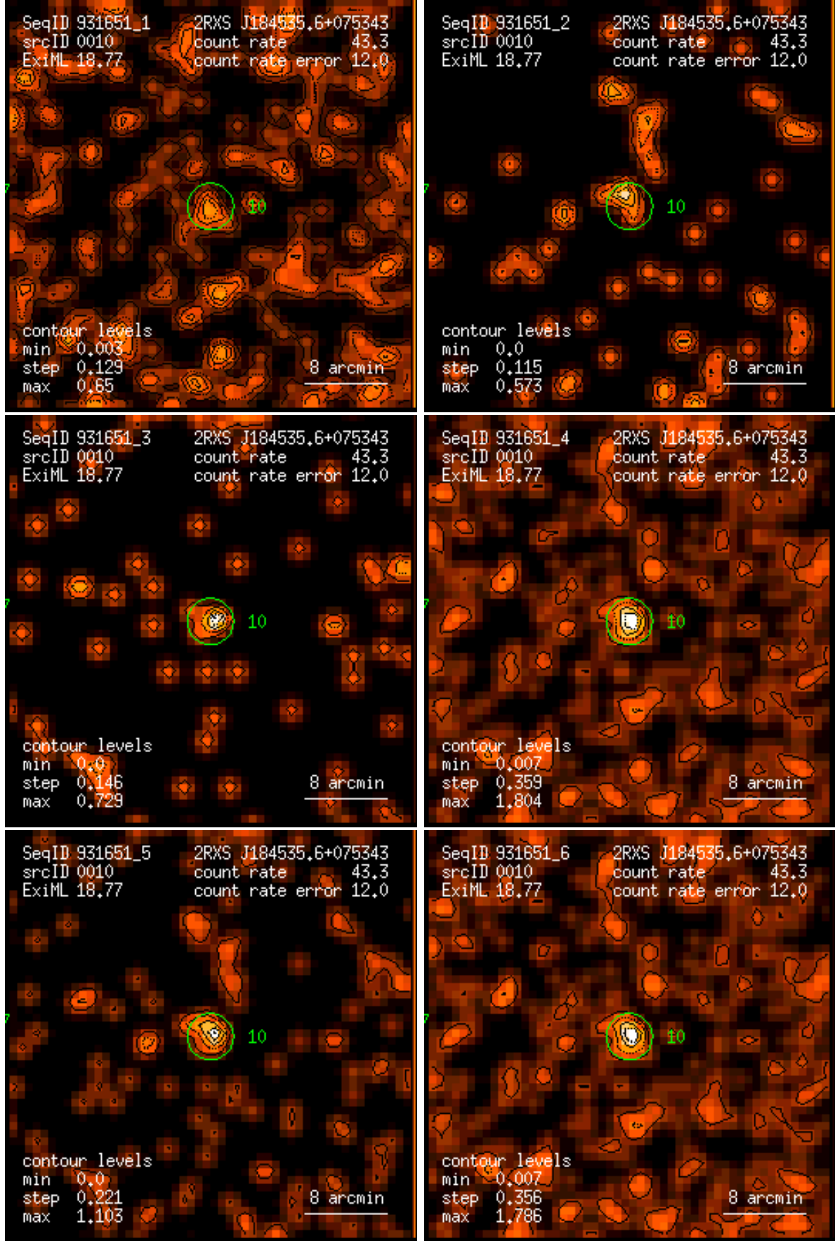
Figure 10: RASS 931651: detection 0010: band rate images, Gaussian filter: (1) PSPC channels 11 – 41, (2) 52 – 90, (3) 91 – 201, (4) 11 – 235, (5) 52 – 201, (6) 11 – 201. Broad band rates in counts/ks. Band rate contour levels in counts/ks/arcmin 2 .
