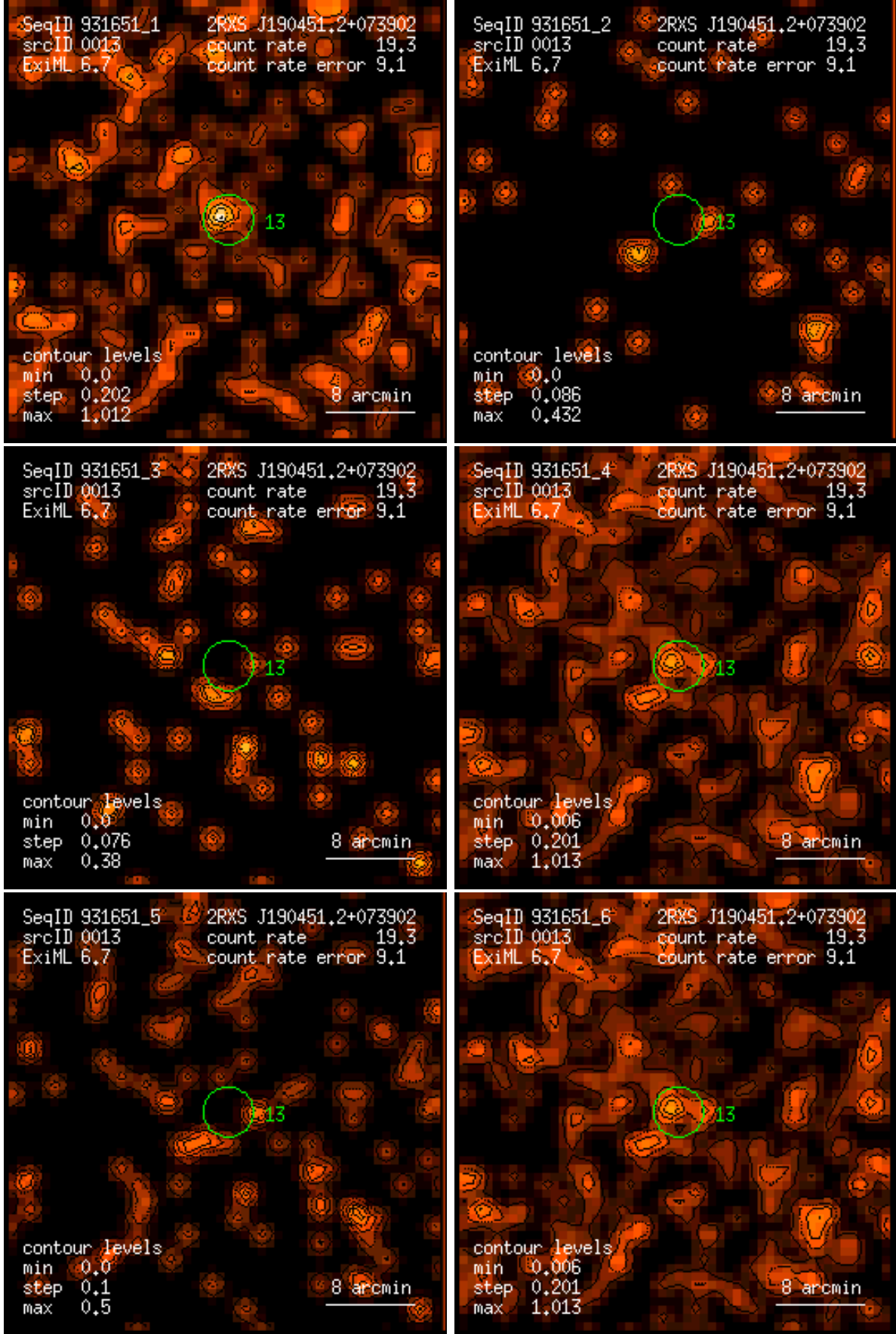
Figure 13: RASS 931651: detection 0013: band rate images, Gaussian filter: (1) PSPC channels 11 – 41, (2) 52 – 90, (3) 91 – 201, (4) 11 – 235, (5) 52 – 201, (6) 11 – 201. Broad band rates in counts/ks. Band rate contour levels in counts/ks/arcmin 2 .
