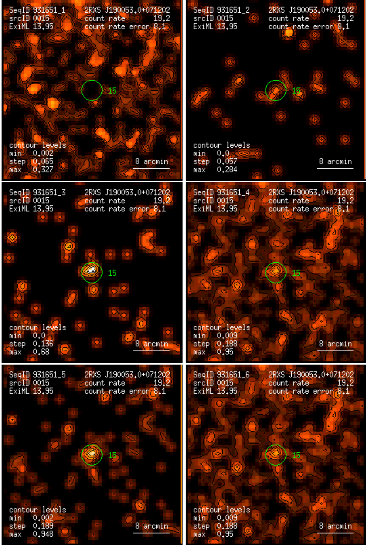
Figure 15: RASS 931651: detection 0015: band rate images, Gaussian filter: (1) PSPC channels 11 – 41, (2) 52 – 90, (3) 91 – 201, (4) 11 – 235, (5) 52 – 201, (6) 11 – 201. Broad band rates in counts/ks. Band rate contour levels in counts/ks/arcmin 2 .
