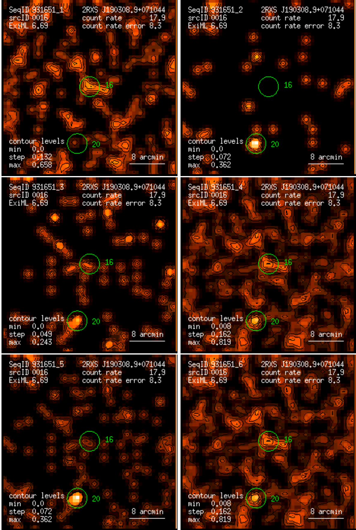
Figure 16: RASS 931651: detection 0016: band rate images, Gaussian filter: (1) PSPC channels 11 – 41, (2) 52 – 90, (3) 91 – 201, (4) 11 – 235, (5) 52 – 201, (6) 11 – 201. Broad band rates in counts/ks. Band rate contour levels in counts/ks/arcmin 2 .
