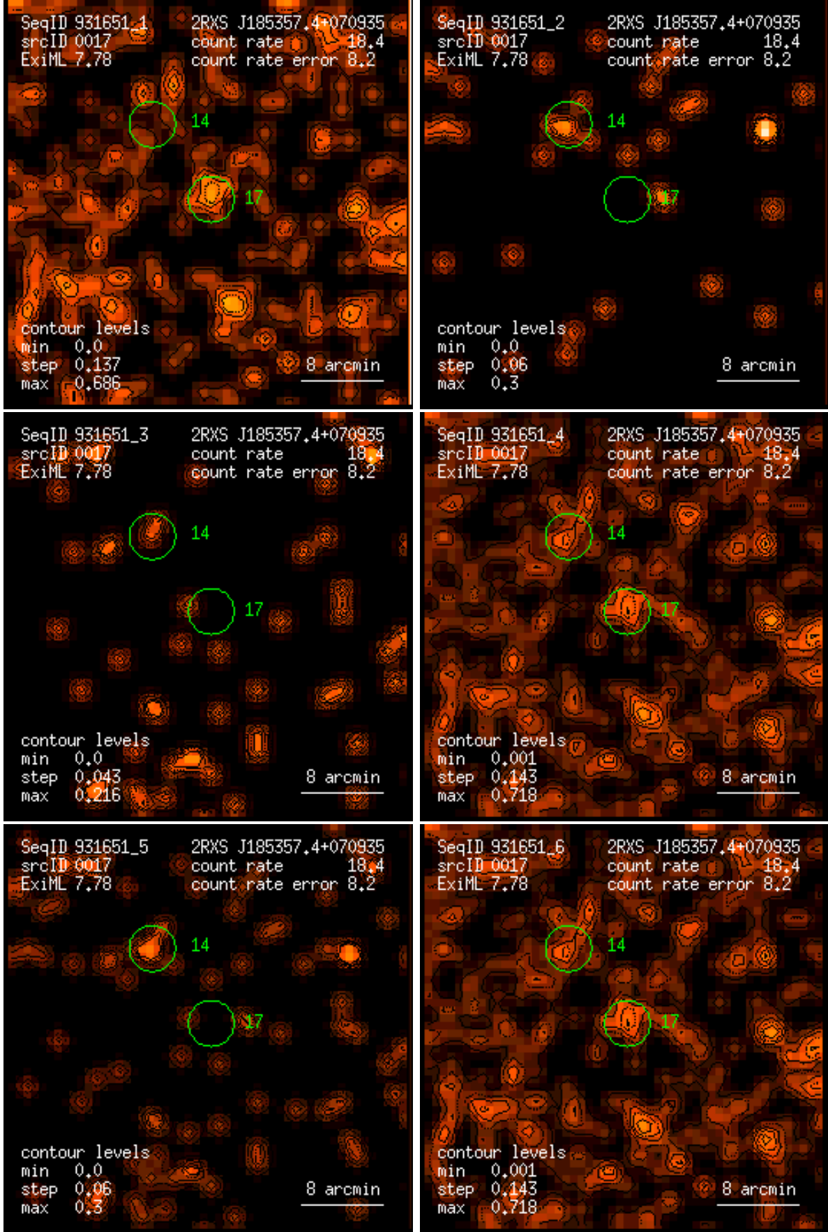
Figure 17: RASS 931651: detection 0017: band rate images, Gaussian filter: (1) PSPC channels 11 – 41, (2) 52 – 90, (3) 91 – 201, (4) 11 – 235, (5) 52 – 201, (6) 11 – 201. Broad band rates in counts/ks. Band rate contour levels in counts/ks/arcmin 2 .
