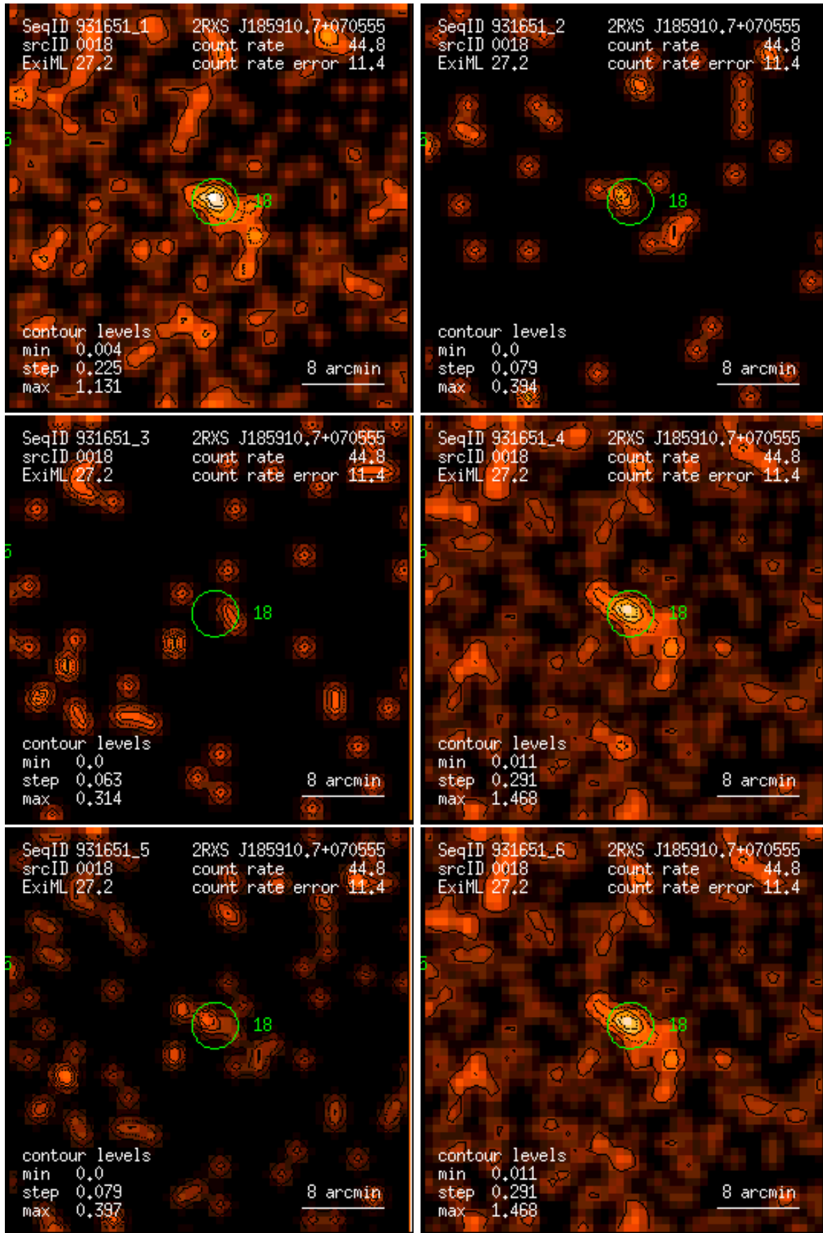
Figure 18: RASS 931651: detection 0018: band rate images, Gaussian filter: (1) PSPC channels 11 – 41, (2) 52 – 90, (3) 91 – 201, (4) 11 – 235, (5) 52 – 201, (6) 11 – 201. Broad band rates in counts/ks. Band rate contour levels in counts/ks/arcmin 2 .
