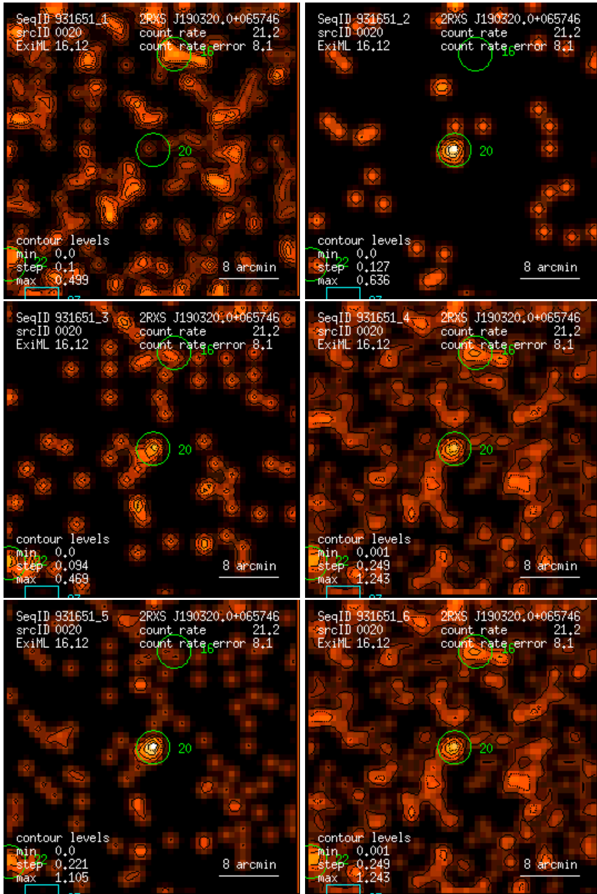
Figure 20: RASS 931651: detection 0020: band rate images, Gaussian filter: (1) PSPC channels 11 – 41, (2) 52 – 90, (3) 91 – 201, (4) 11 – 235, (5) 52 – 201, (6) 11 – 201. Broad band rates in counts/ks. Band rate contour levels in counts/ks/arcmin 2 .
