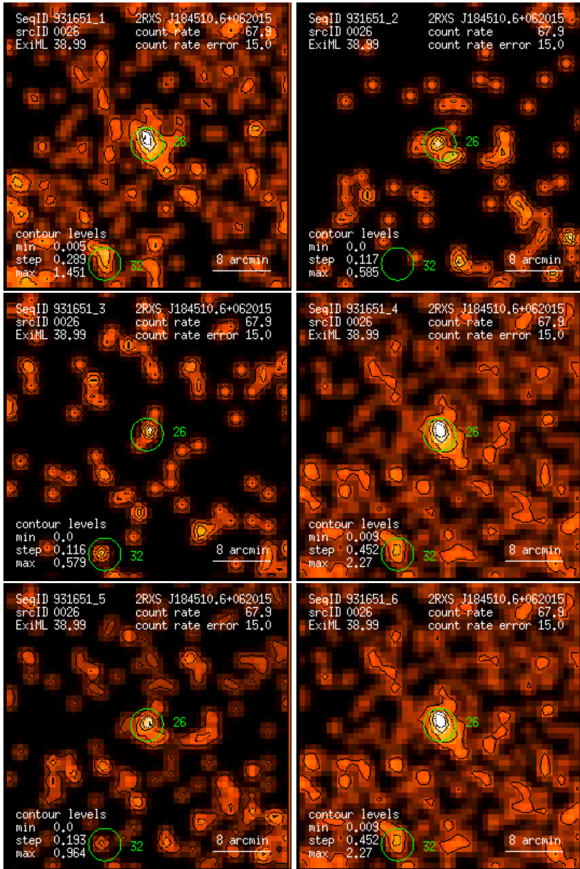
Figure 26: RASS 931651: detection 0026: band rate images, Gaussian filter: (1) PSPC channels 11 – 41, (2) 52 – 90, (3) 91 – 201, (4) 11 – 235, (5) 52 – 201, (6) 11 – 201. Broad band rates in counts/ks. Band rate contour levels in counts/ks/arcmin 2 .
