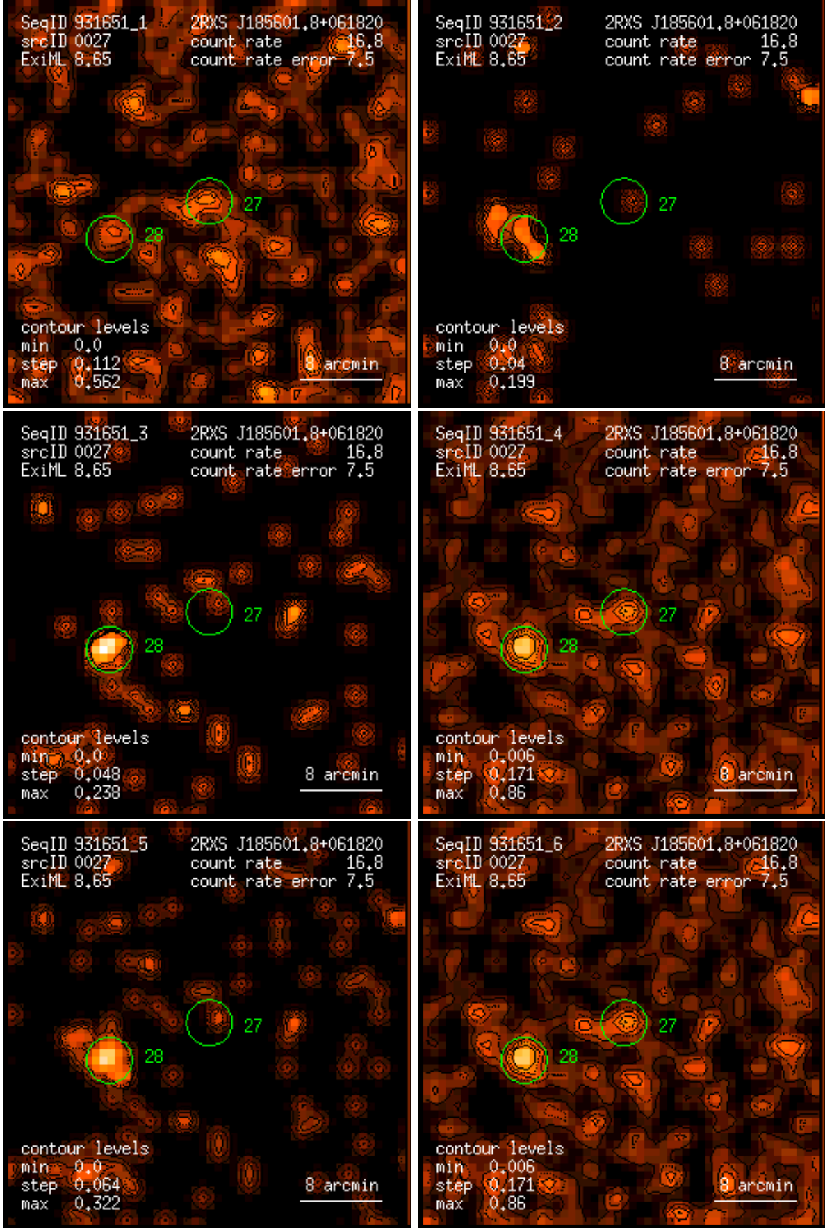
Figure 27: RASS 931651: detection 0027: band rate images, Gaussian filter: (1) PSPC channels 11 – 41, (2) 52 – 90, (3) 91 – 201, (4) 11 – 235, (5) 52 – 201, (6) 11 – 201. Broad band rates in counts/ks. Band rate contour levels in counts/ks/arcmin 2 .
