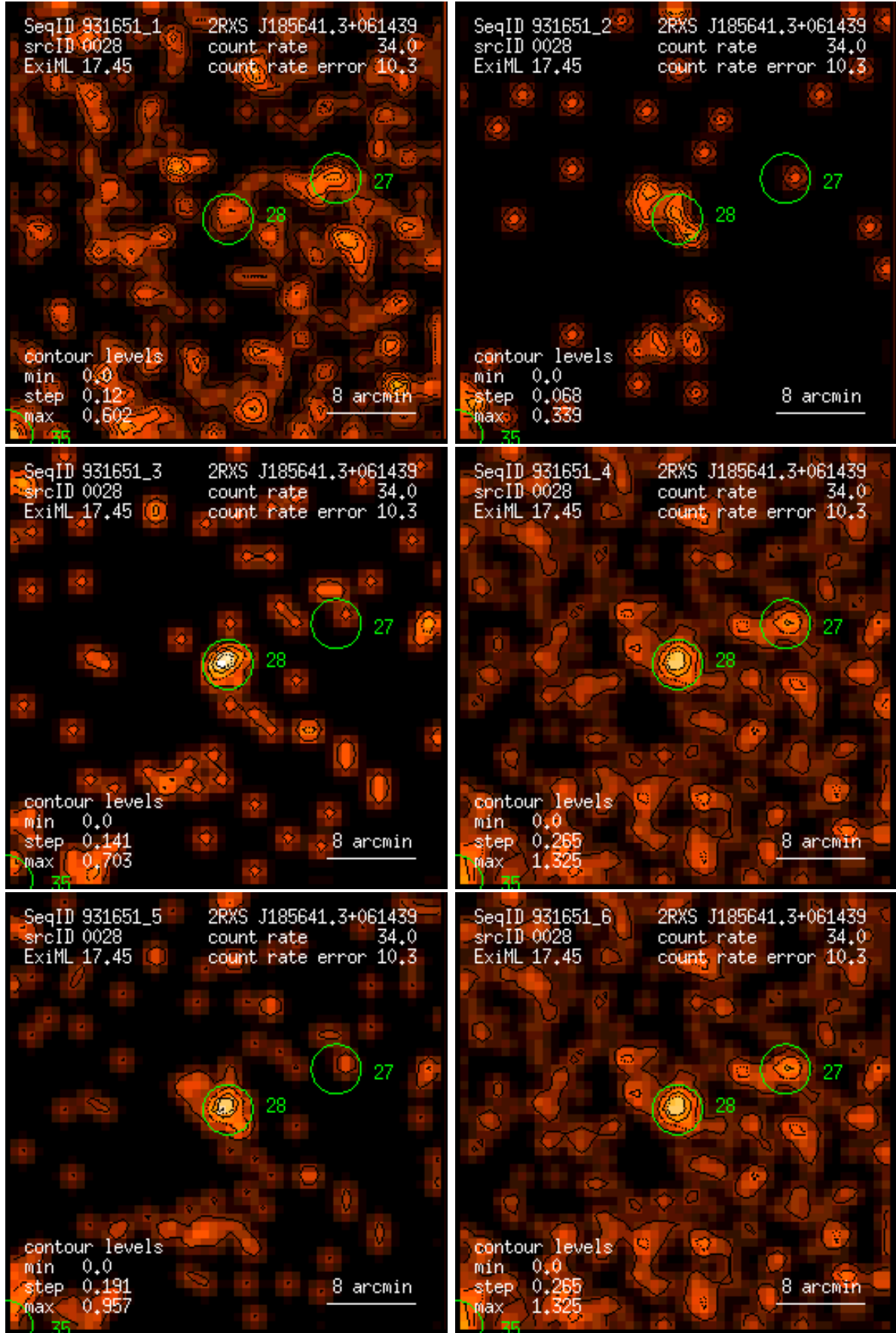
Figure 28: RASS 931651: detection 0028: band rate images, Gaussian filter: (1) PSPC channels 11 – 41, (2) 52 – 90, (3) 91 – 201, (4) 11 – 235, (5) 52 – 201, (6) 11 – 201. Broad band rates in counts/ks. Band rate contour levels in counts/ks/arcmin 2 .
