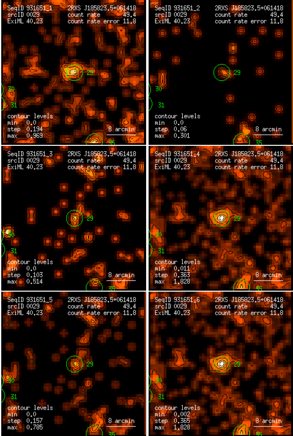
Figure 29: RASS 931651: detection 0029: band rate images, Gaussian filter: (1) PSPC channels 11 – 41, (2) 52 – 90, (3) 91 – 201, (4) 11 – 235, (5) 52 – 201, (6) 11 – 201. Broad band rates in counts/ks. Band rate contour levels in counts/ks/arcmin 2 .
