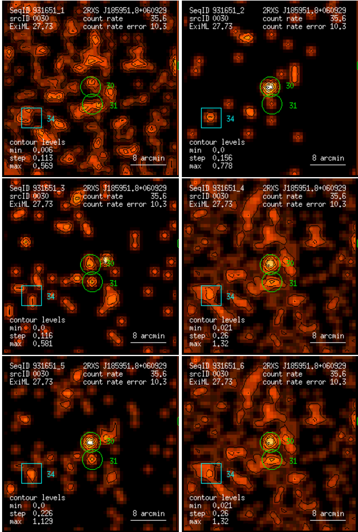
Figure 30: RASS 931651: detection 0030: band rate images, Gaussian filter: (1) PSPC channels 11 – 41, (2) 52 – 90, (3) 91 – 201, (4) 11 – 235, (5) 52 – 201, (6) 11 – 201. Broad band rates in counts/ks. Band rate contour levels in counts/ks/arcmin 2 .
