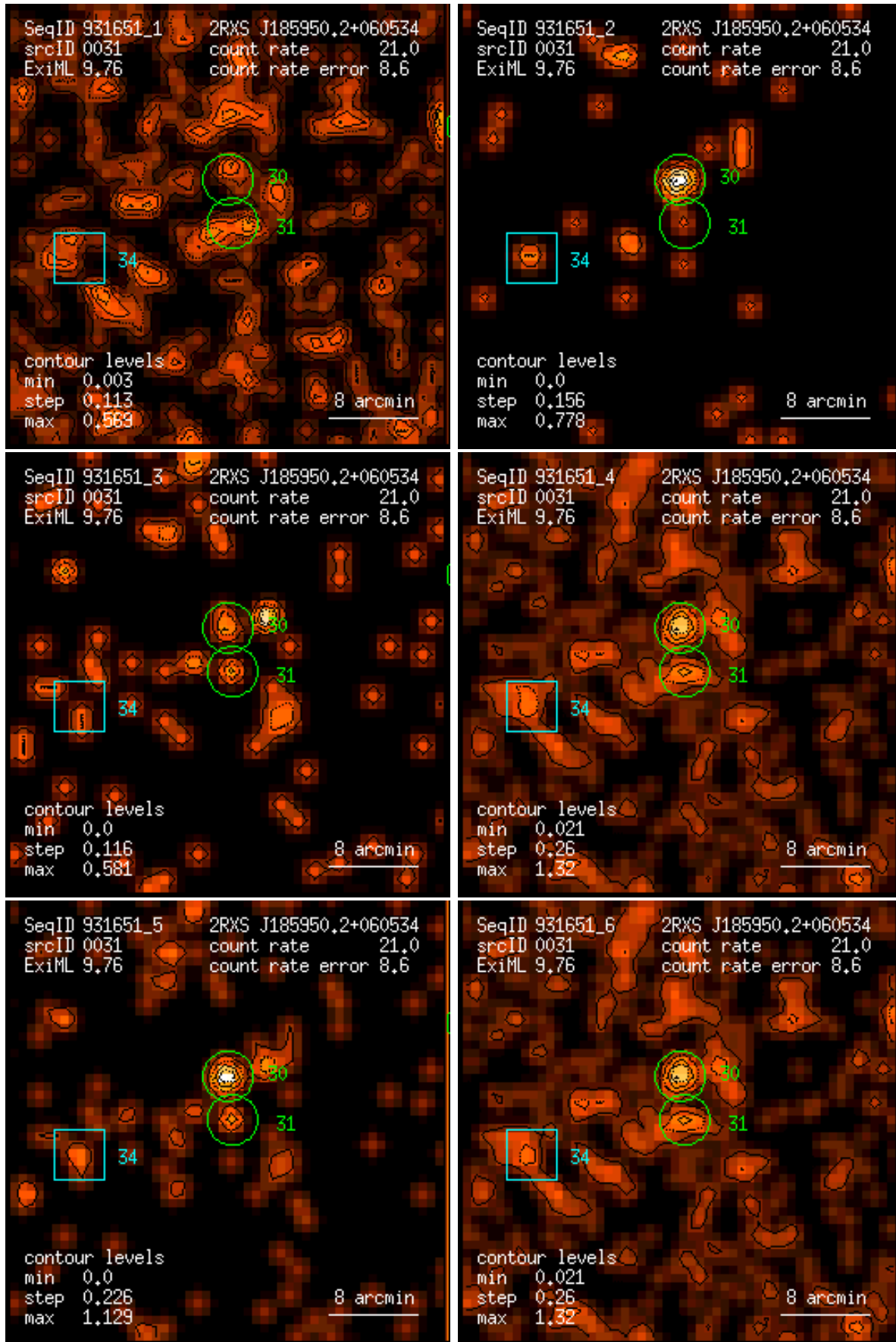
Figure 31: RASS 931651: detection 0031: band rate images, Gaussian filter: (1) PSPC channels 11 – 41, (2) 52 – 90, (3) 91 – 201, (4) 11 – 235, (5) 52 – 201, (6) 11 – 201. Broad band rates in counts/ks. Band rate contour levels in counts/ks/arcmin 2 .
