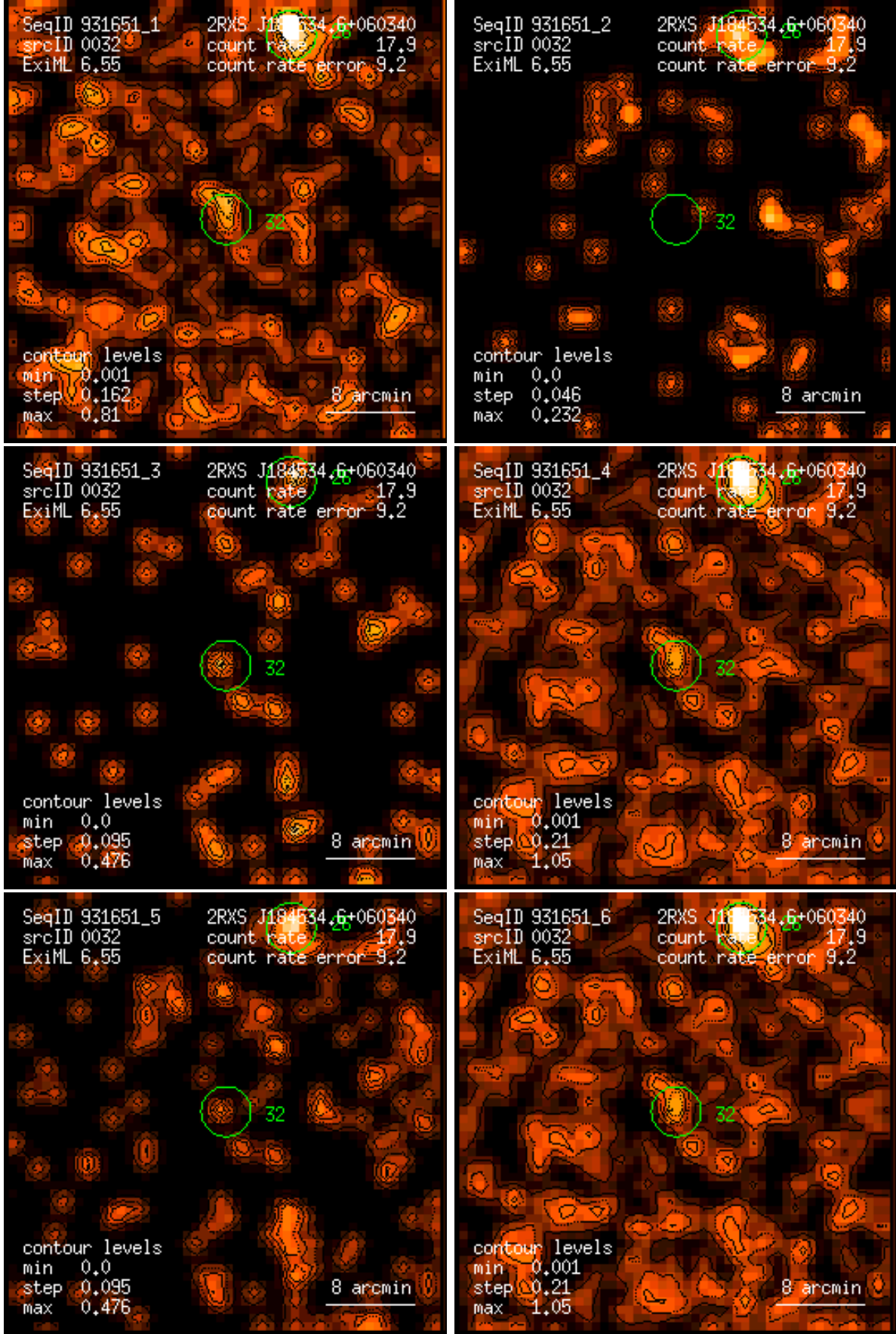
Figure 32: RASS 931651: detection 0032: band rate images, Gaussian filter: (1) PSPC channels 11 – 41, (2) 52 – 90, (3) 91 – 201, (4) 11 – 235, (5) 52 – 201, (6) 11 – 201. Broad band rates in counts/ks. Band rate contour levels in counts/ks/arcmin 2 .
