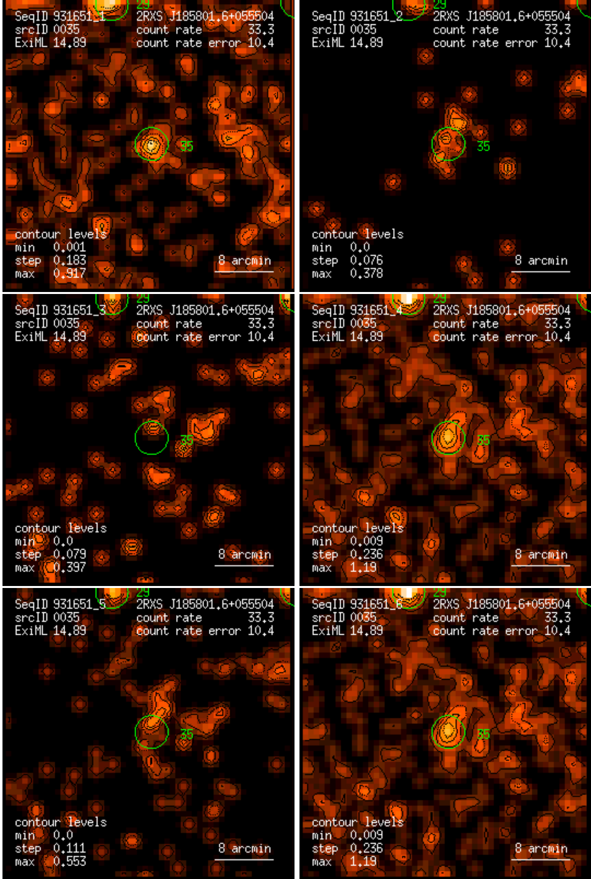
Figure 35: RASS 931651: detection 0035: band rate images, Gaussian filter: (1) PSPC channels 11 – 41, (2) 52 – 90, (3) 91 – 201, (4) 11 – 235, (5) 52 – 201, (6) 11 – 201. Broad band rates in counts/ks. Band rate contour levels in counts/ks/arcmin 2 .
