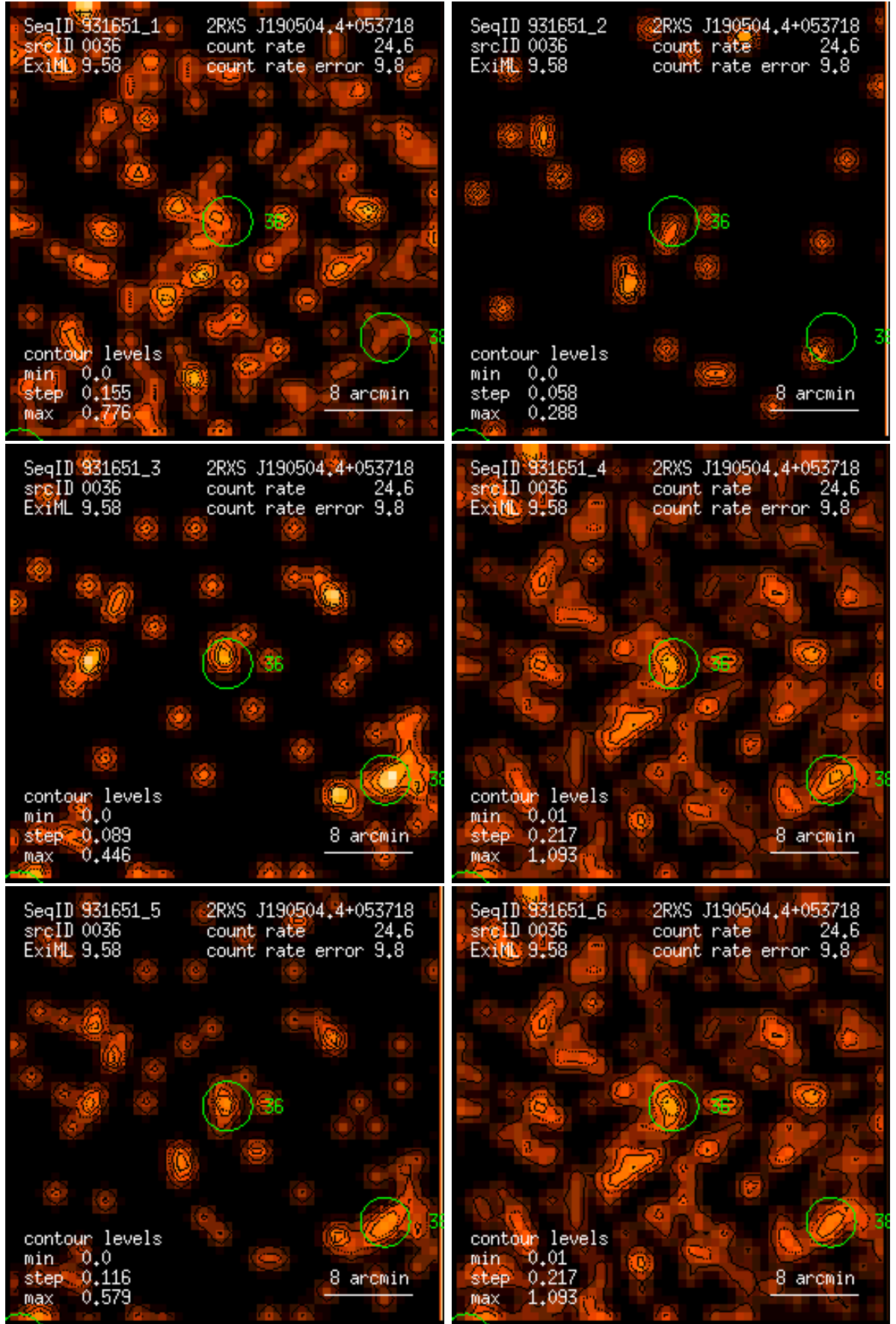
Figure 36: RASS 931651: detection 0036: band rate images, Gaussian filter: (1) PSPC channels 11 – 41, (2) 52 – 90, (3) 91 – 201, (4) 11 – 235, (5) 52 – 201, (6) 11 – 201. Broad band rates in counts/ks. Band rate contour levels in counts/ks/arcmin 2 .
