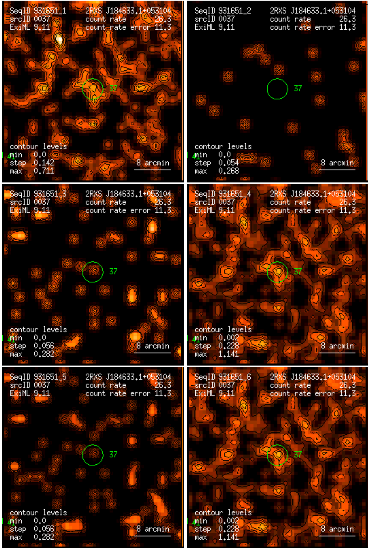
Figure 37: RASS 931651: detection 0037: band rate images, Gaussian filter: (1) PSPC channels 11 – 41, (2) 52 – 90, (3) 91 – 201, (4) 11 – 235, (5) 52 – 201, (6) 11 – 201. Broad band rates in counts/ks. Band rate contour levels in counts/ks/arcmin 2 .
