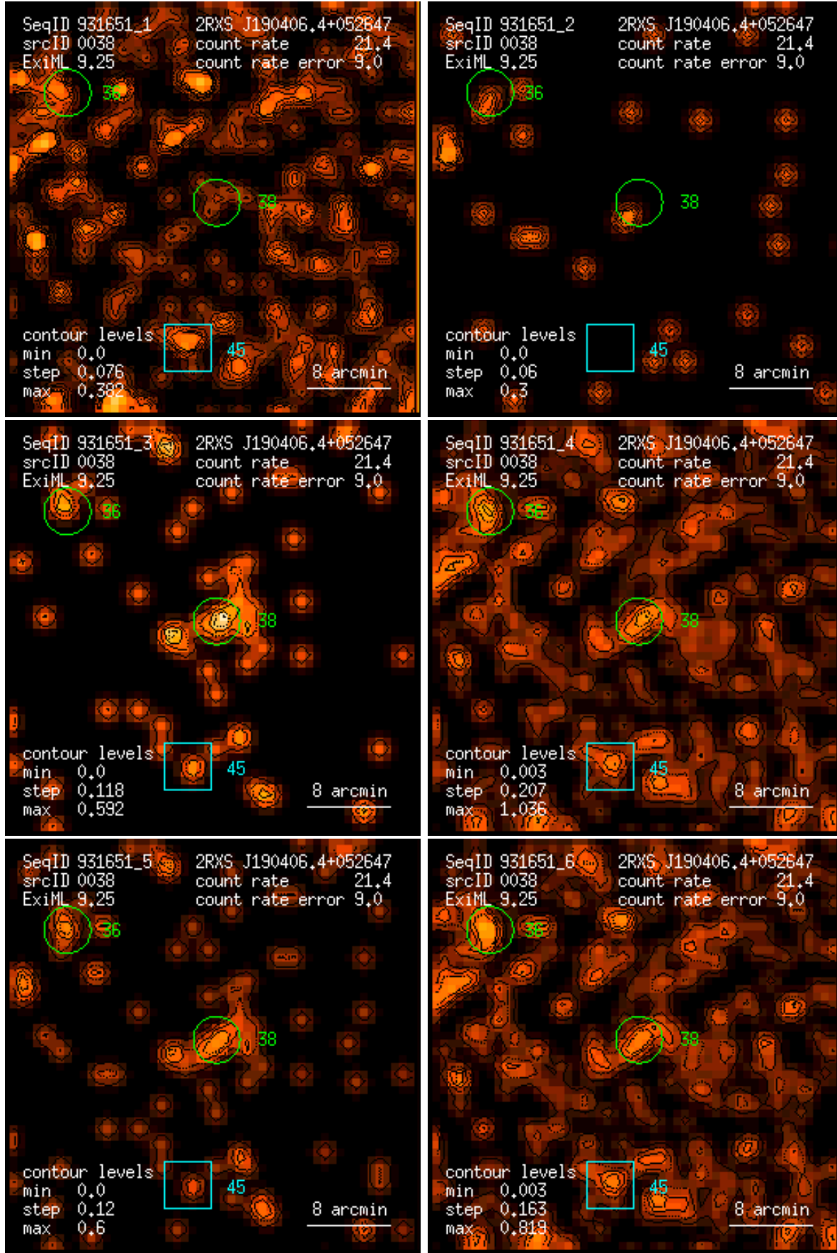
Figure 38: RASS 931651: detection 0038: band rate images, Gaussian filter: (1) PSPC channels 11 – 41, (2) 52 – 90, (3) 91 – 201, (4) 11 – 235, (5) 52 – 201, (6) 11 – 201. Broad band rates in counts/ks. Band rate contour levels in counts/ks/arcmin 2 .
